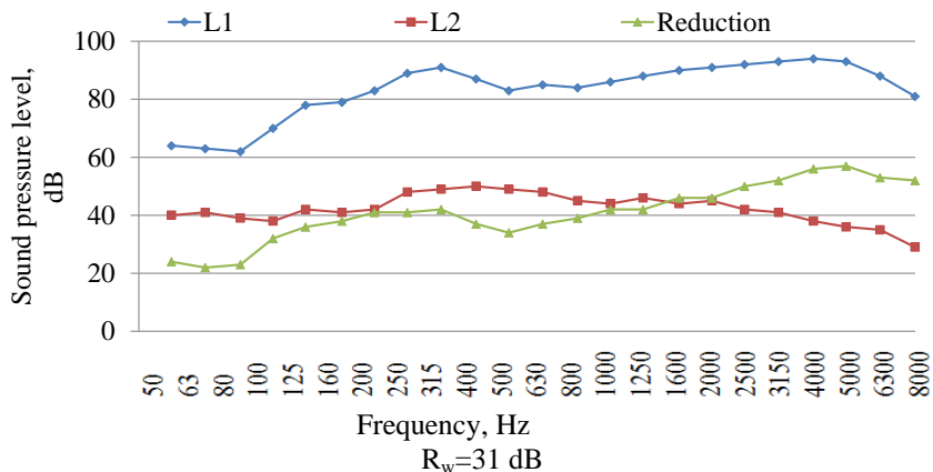
Fig. 7. Sound pressure level difference. construction with shredded tire chips and concrete with a mixture of concave surface results. The sound pressure level is sent to the L1, L2, sound pressure level for the wall
