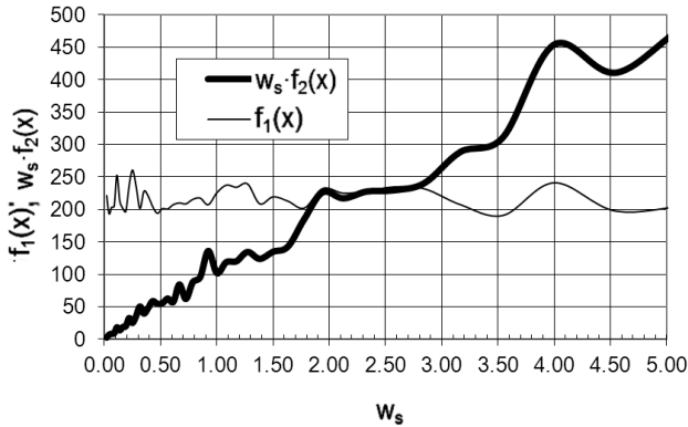
Fig. 4. Contribution of components of the objective function to optimization solution (15 pile grillage)
