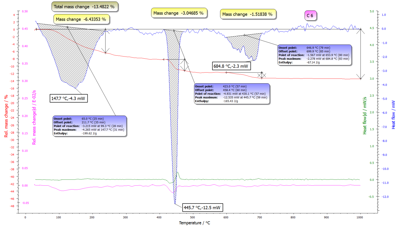
Fig. D.2. Simultaneous thermal analysis for cement paste modified by 0.06 % bwoc of MWCNT
