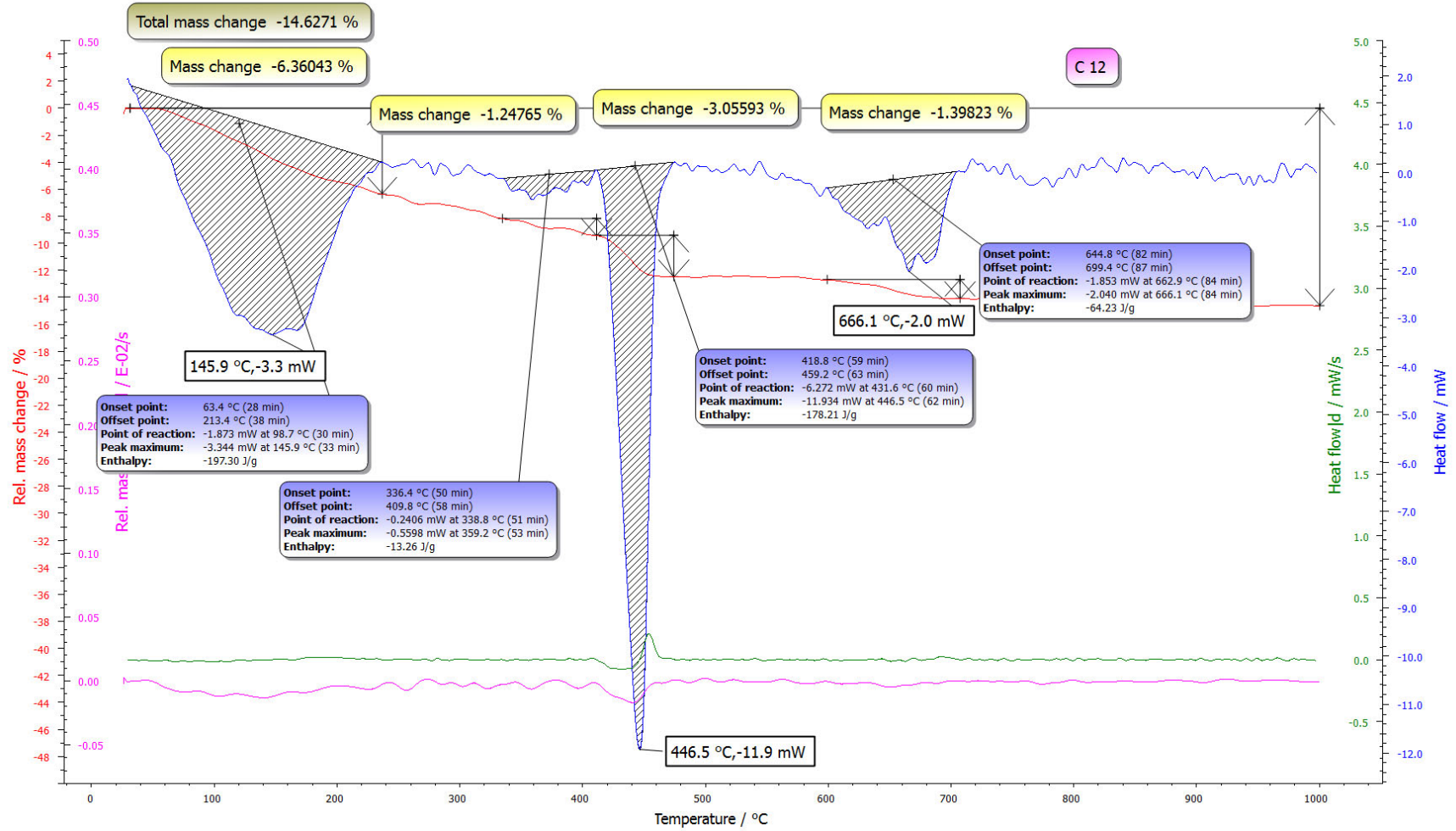
Fig. D.3. Simultaneous thermal analysis for cement paste modified by 0.12 % bwoc of MWCNT
