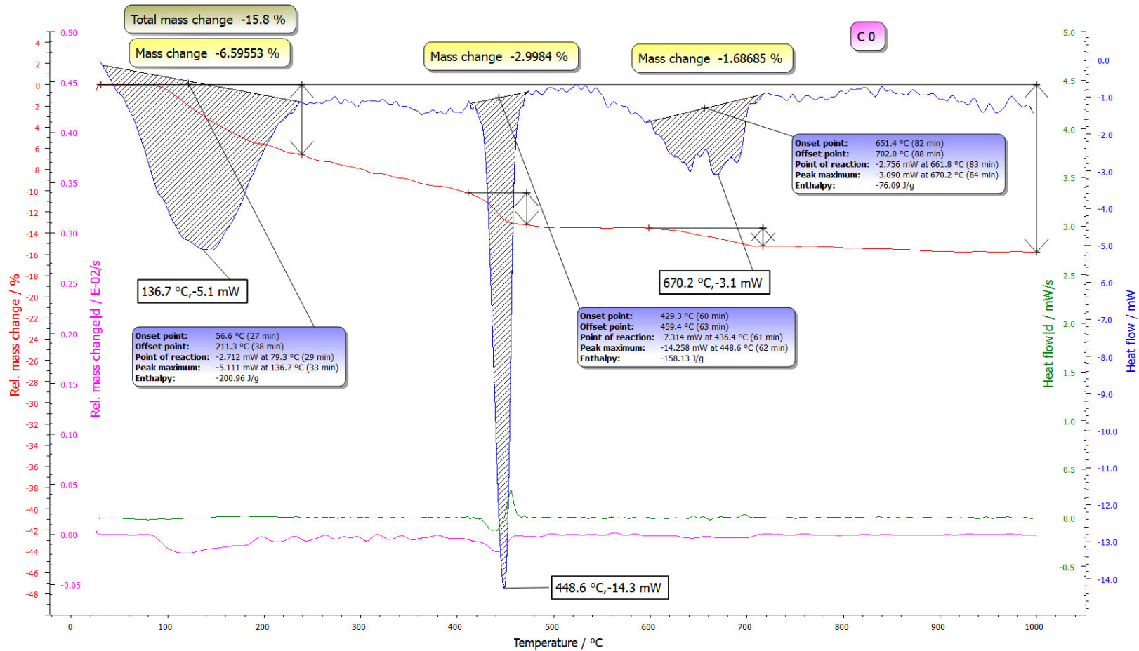
Fig. D.1. Simultaneous thermal analysis for cement paste without admixtures (reference)
