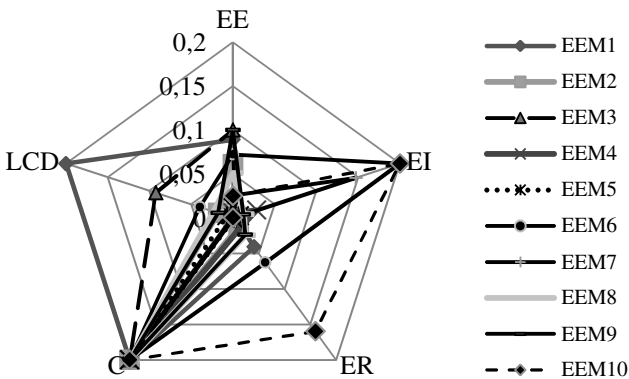
Fig. 3. Sustainability criteria of separate energy efficiency measures of building A
