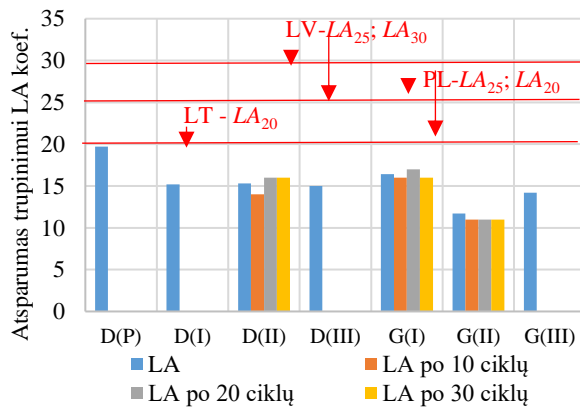
F.2 pav. Atsparumas trupinimui (Los Andželo koeficientas) ( LA ) Fig. F.2. Resistance to fragmentation (Los Angeles coefficient) ( LA )
