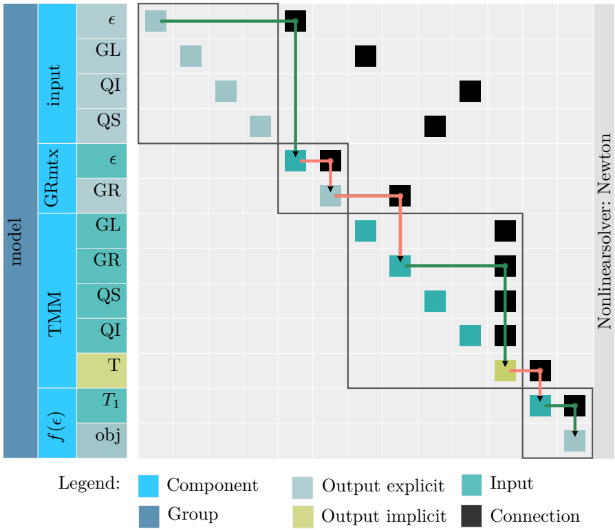
Fig. D.2. N2 diagram of the CubeSat optimization model in OpenMDAO
