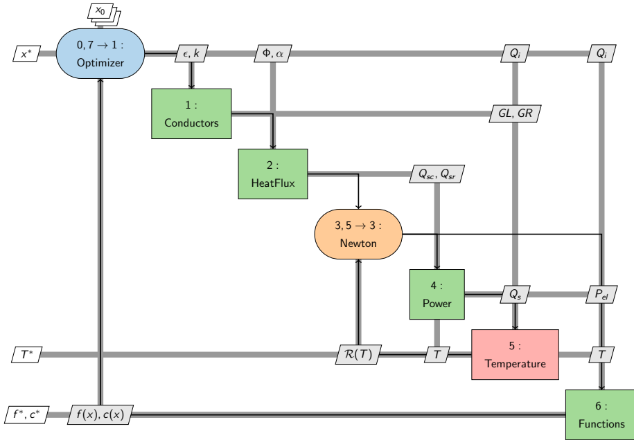
Fig. D.1. XDSM diagram for MAT optimization problem. The data flow in the figure is shown as thick gray lines. Components take data inputs from the vertical direction and output data in the horizontal direction. The thin black lines show the process flow, with numbers showing the order in which the components are executed.
