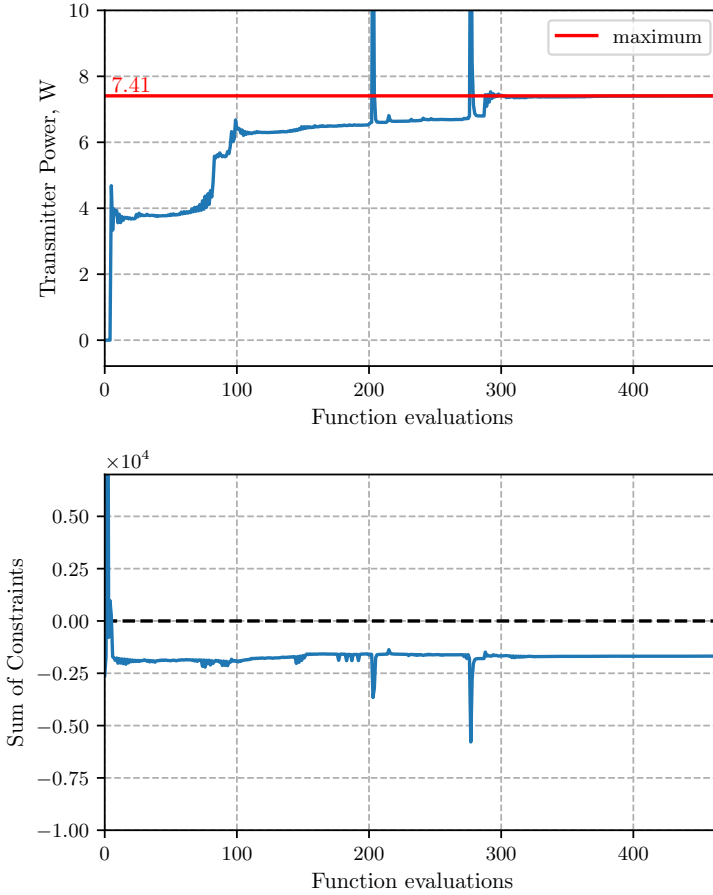
Fig. C.2. Optimization convergence history of MS uncoupled model. Total run time on Intel Core i5-5300U processor: 5530 s.
