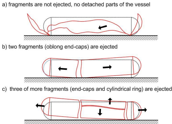
Fig. 1 Probable fragmentation patterns of an unconstrained vessel (e.g., vessel of a road or railway tanker involved in a traffic accident)
