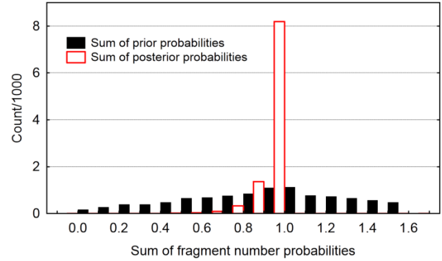
Fig. 6 Histograms of the samples \varepsilon and \varepsilon' consisting of simulated sums of the prior and posterior fragment number probabilities p_i(n_{frg}) and p'_i(n_{frg})
