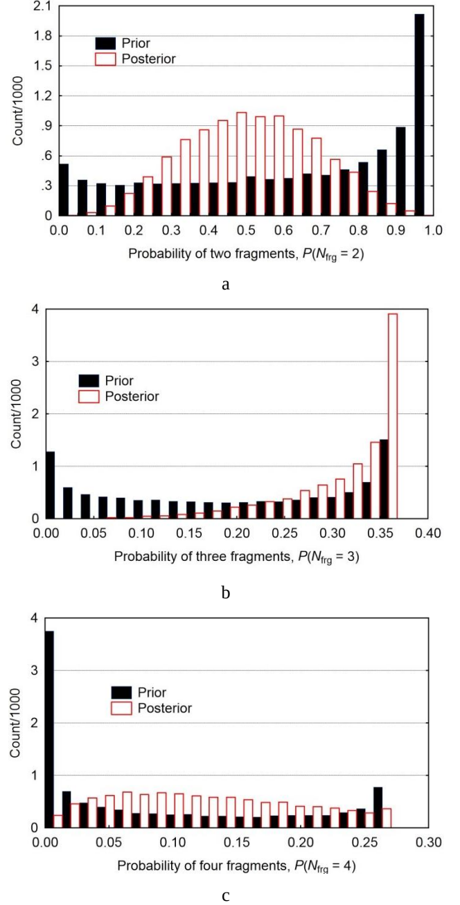
Fig. 5 Histograms of the sample pairs (\mathbf{p}_m, \mathbf{p}'_m) generated to assess prior and posterior uncertainty in the fragment number probabilities P(N_{frag} = m) : a) the case m = 2 ; b) the case m = 3 ; c) the case m = 4
