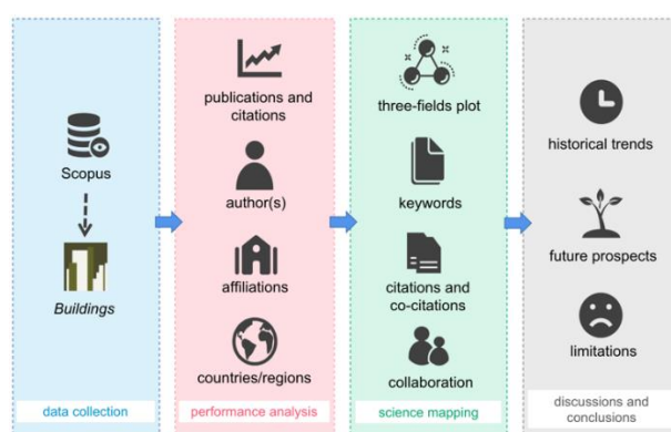
Figure 1. The process of bibliometric analysis.
