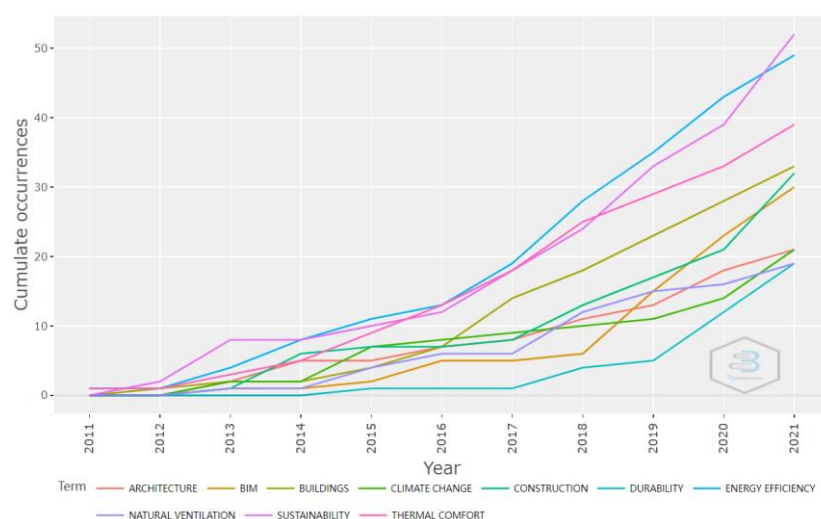
Figure 5. Growth of the top 10 keywords.
