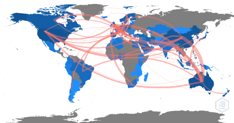
Figure 12. An overview of cooperation between countries/regions.
