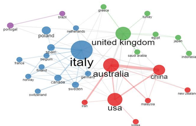
Figure 13. Collaboration network of countries/regions.
