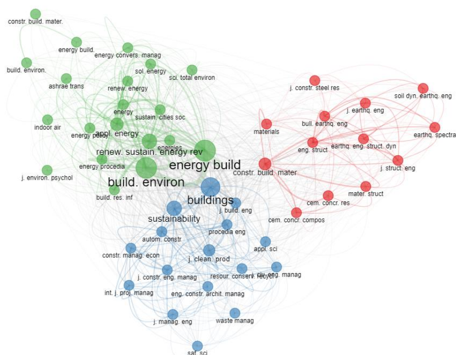
Figure 10. Co-citation network of journals.
