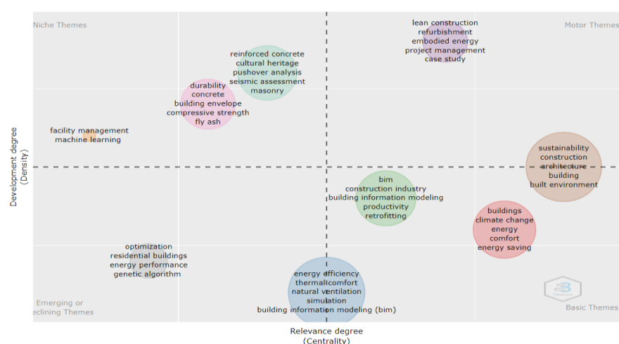
Figure 4. Thematic map of keywords.
