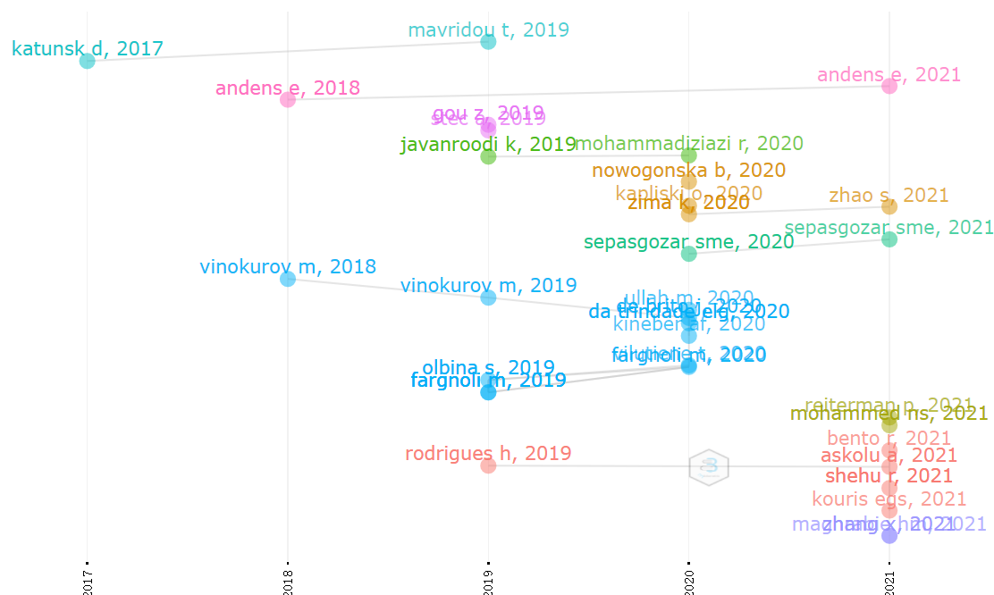
Figure 9. Historical direct citation network.
