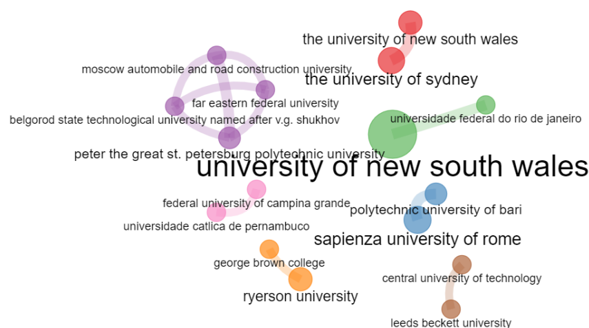
Figure 11. Collaboration network of institutions.
