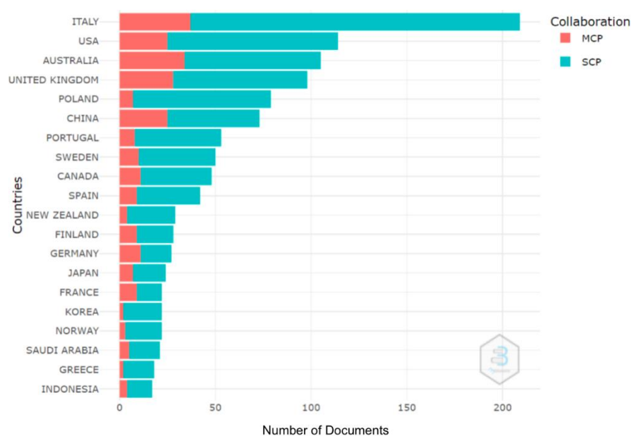
Figure 2. Most productive countries/regions.
