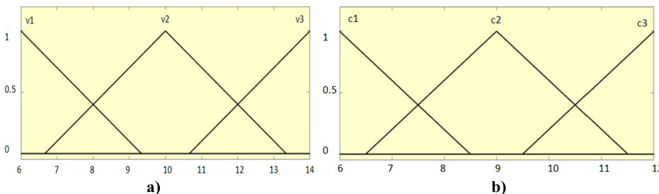
Fig. 6. The inputs: a) PV voltage ( I_{PV} ) MFs; b) PV current ( P_{PV} ) MFs.
