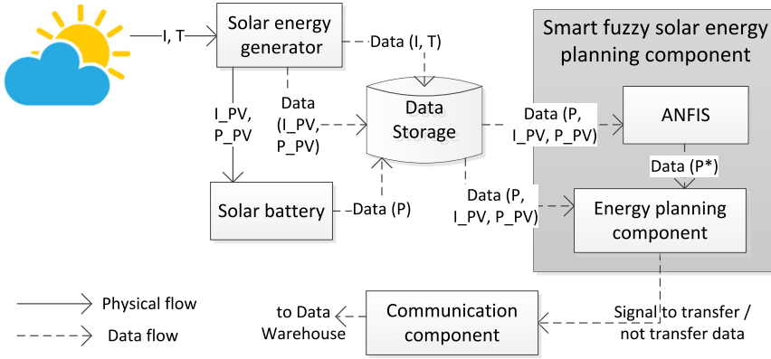
Fig. 3. The proposed Smart-Sole (I – Irradiation (W/m 2 ), T – Temperature, °C, P – power, W, generated by Solar energy generator, P* – power, W, predicted by ANFIS, I_PV – current, A, P_PV – voltage, V).
