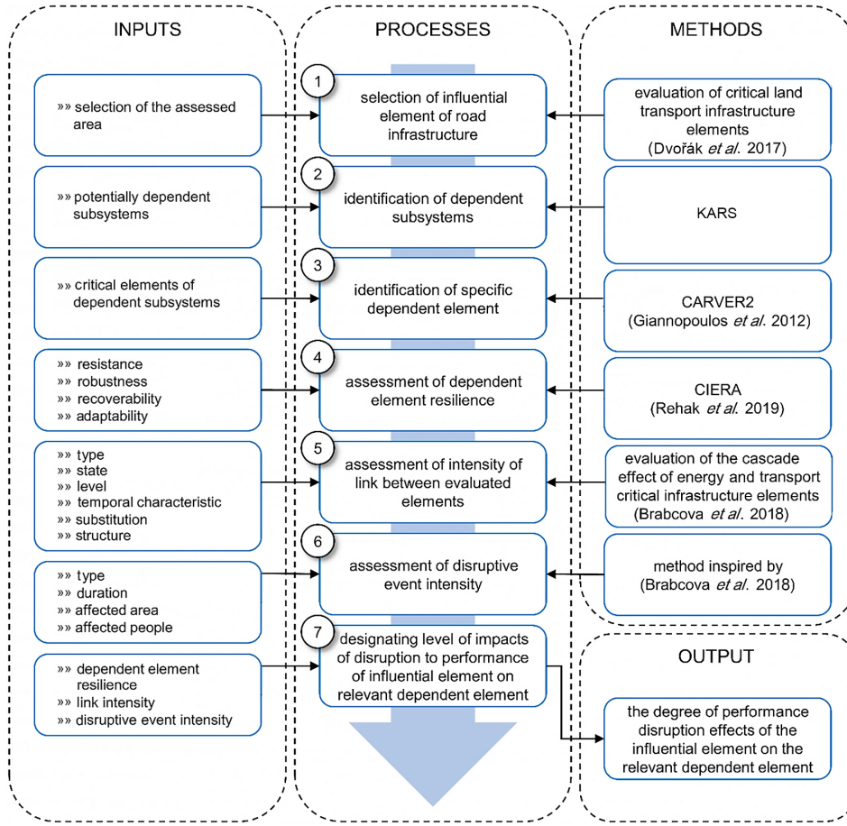
Figure 3. A comprehensive approach to assessing impacts of disruption to performance of road infrastructure elements on dependent subsystems
