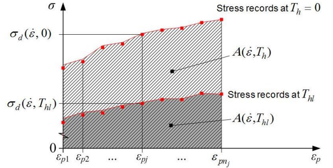
Fig. 5 An illustration of the areas below true stress versus true strain records, A(\dot{\varepsilon}, T_{hl}) and A(\dot{\varepsilon}, T_h) , obtained at the temperatures T_{hl} and T_h
