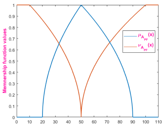
Figure A1. Graphical representation of membership functions of Pythagorean fuzzy set.
