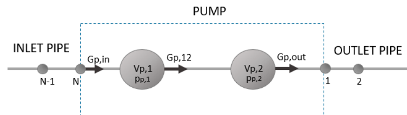
Figure 5. High-pressure booster pump mathematical model. Note: N, N-1—numbers of inlet pipe sections; 1, 2—numbers of outlet pipe sections; Vp,1—the passage between the pipe and the first stage of pump’s joint; Vp,2—the passage between the pipe and the second stage of pump’s joint; Gp—mass flow of LNG.
