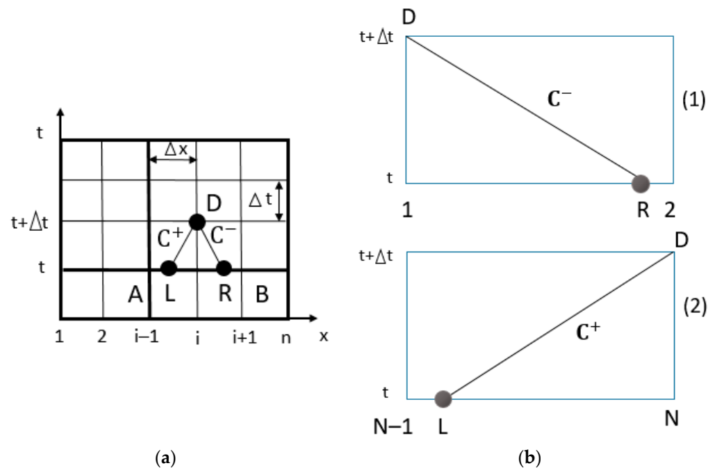
Figure 6. Method of characteristics (a) Schematic of characteristic line for MOC; (b) Calculation schemes of the first and the last points.
