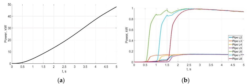
Figure 16. Hydraulic energy losses. Note: (a) Hydraulic energy losses in the 1st pipeline (L1); (b) Hydraulic energy losses in all pipelines and pipes.
