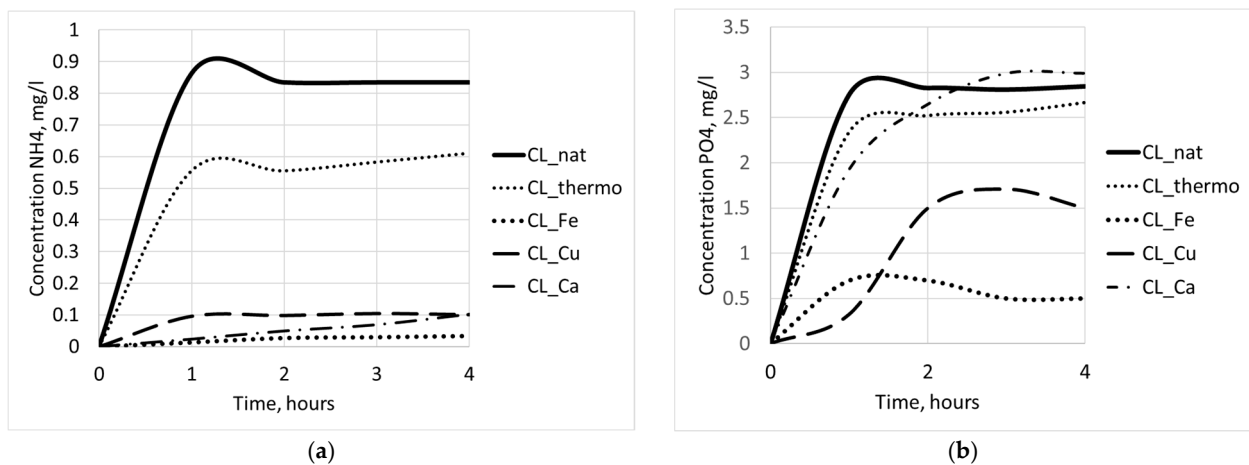
Figure 6. Breakthrough curves: (a)— \text{NH}_4^+ ; (b)— \text{PO}_4^{3-} .
