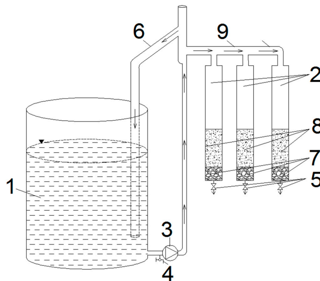
Figure 1. Scheme of the experimental stand: 1—wastewater tank, 2—filtration columns, 3—supply pump, 4—sampling point (before filtration), 5—filtrate collection point, 6—overflow tube, 7—retaining layer, 8—filter media, and 9—wastewater distribution pipe to columns.
