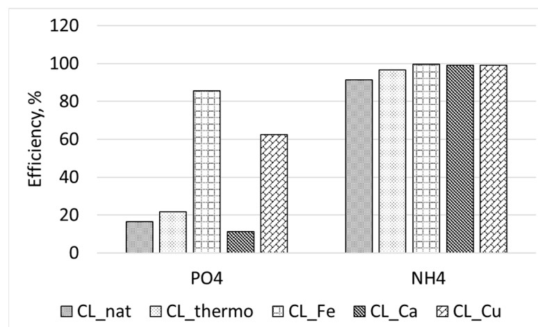
Figure 7. The efficiency of treatment.
