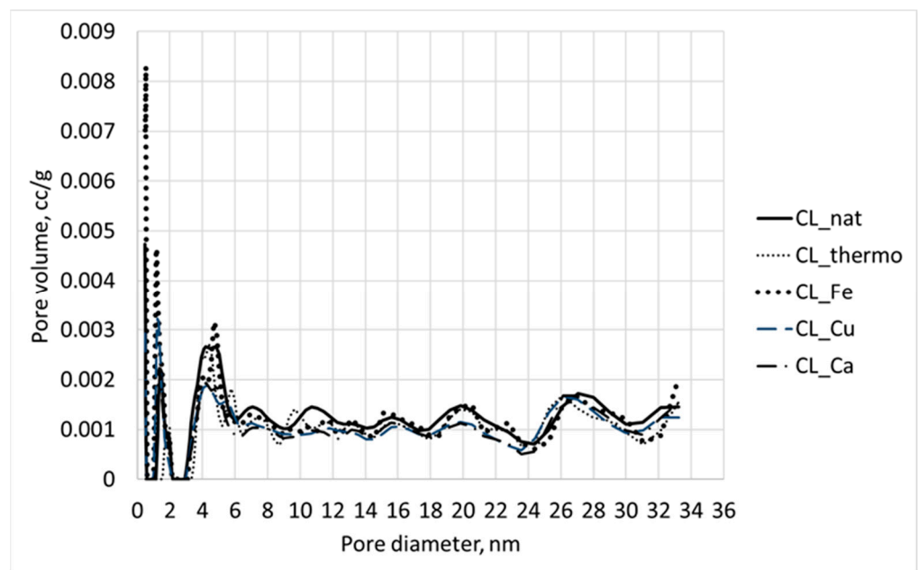
Figure 3. Pore size distribution.
