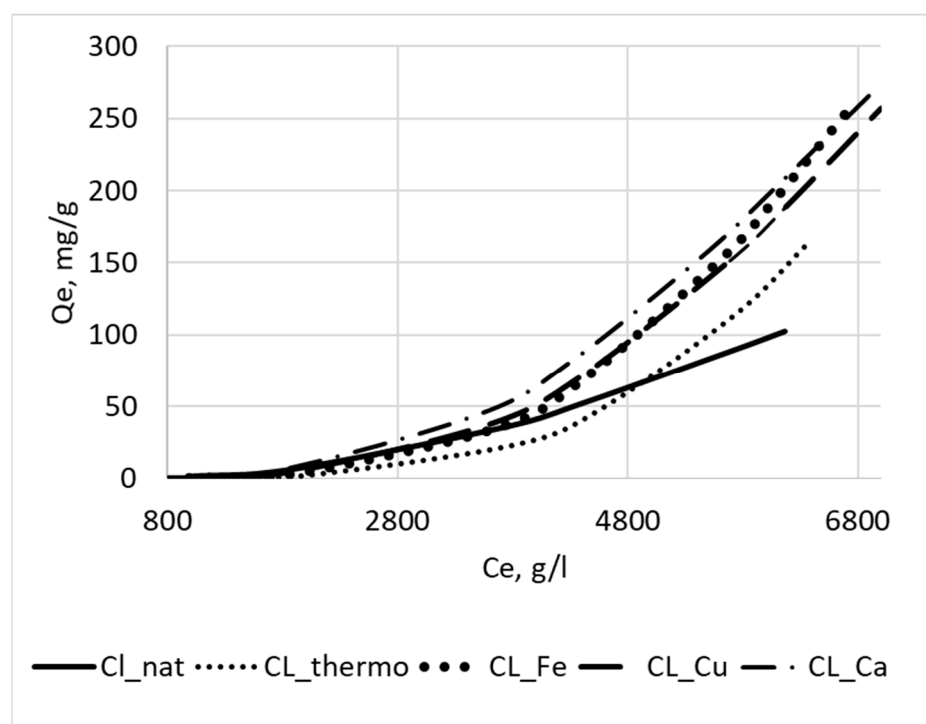
Figure 5. Isotherms of PO 4 3- adsorption.
