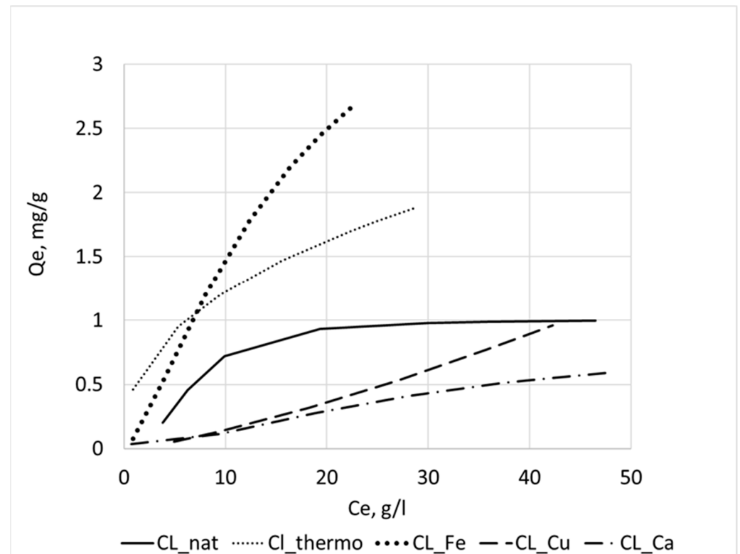
Figure 4. Isotherms of \text{NH}_4^+ adsorption.
