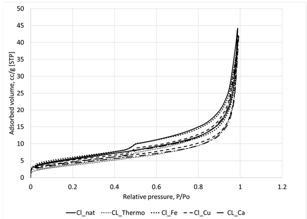
Figure 2. N 2 adsorption–desorption isotherms.
