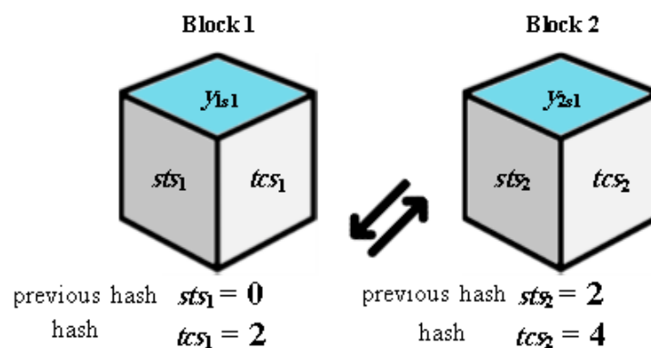
Figure 12. The linkage between blocks.
