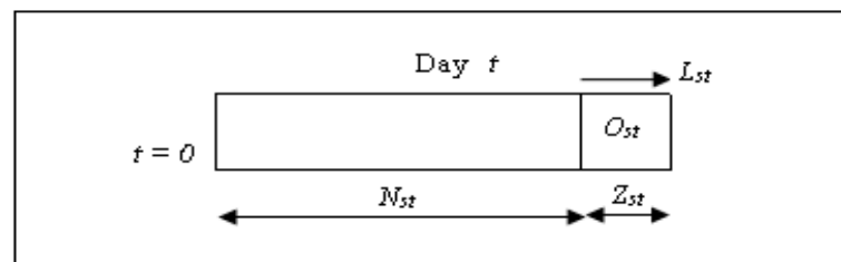
Figure 7. Illustration of closing time for shop s .
