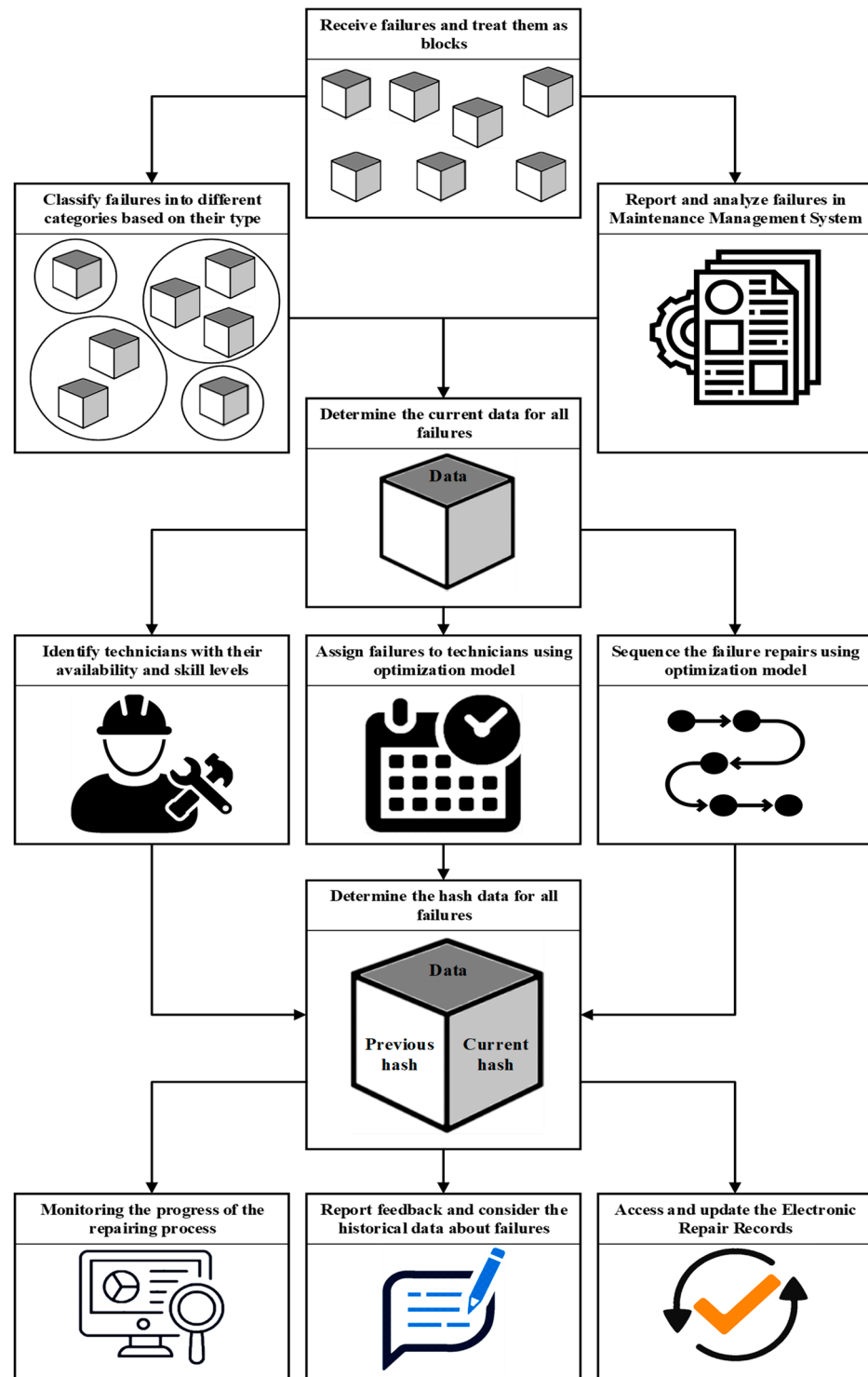
Figure 3. The life cycle of the ERR system.
