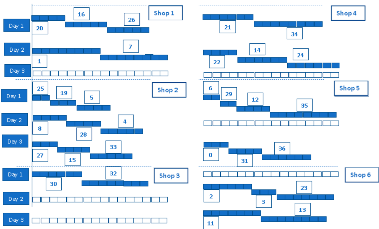
Figure 16. The sequencing repairs for the scheduled failures.
