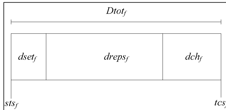
Figure 8. Illustration of related times of failure f .
