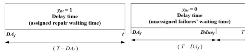
Figure 5. Illustration of delay time calculation.
