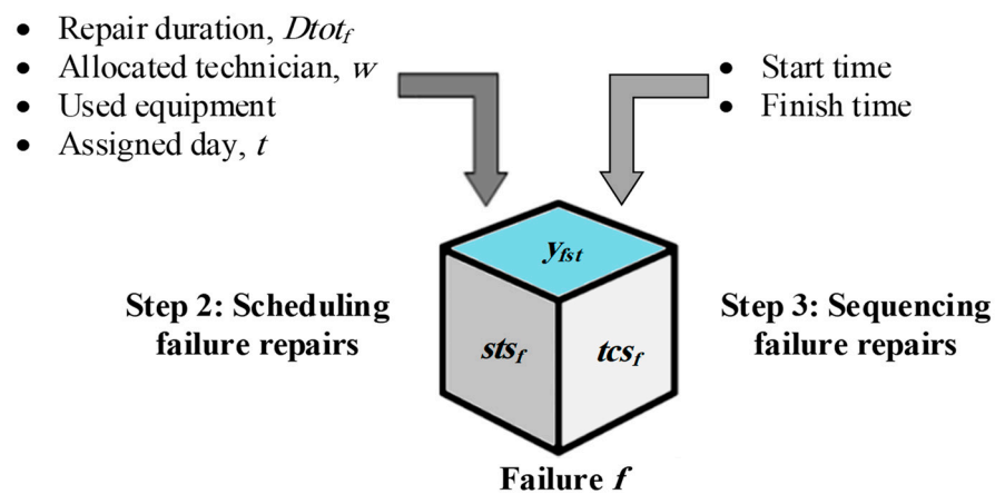
Figure 11. The stored data in each block after step 3.
