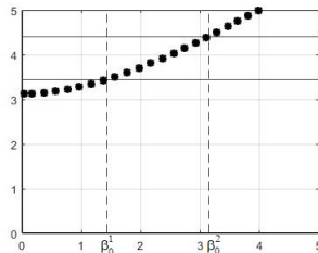
Figure 8. Graphics of the function f(\beta, \xi) for \xi = 0.6 . If \gamma_2 > \gamma_1 , then \beta_0^2 > \beta_0^1 .
