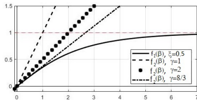
Figure 3. Graphics of the function f_1(\beta) for \xi = 0.5 and function f_2(\beta) for h = 0.02 and various \gamma . The root \beta_0 of Equation (2.8) does not exist.
