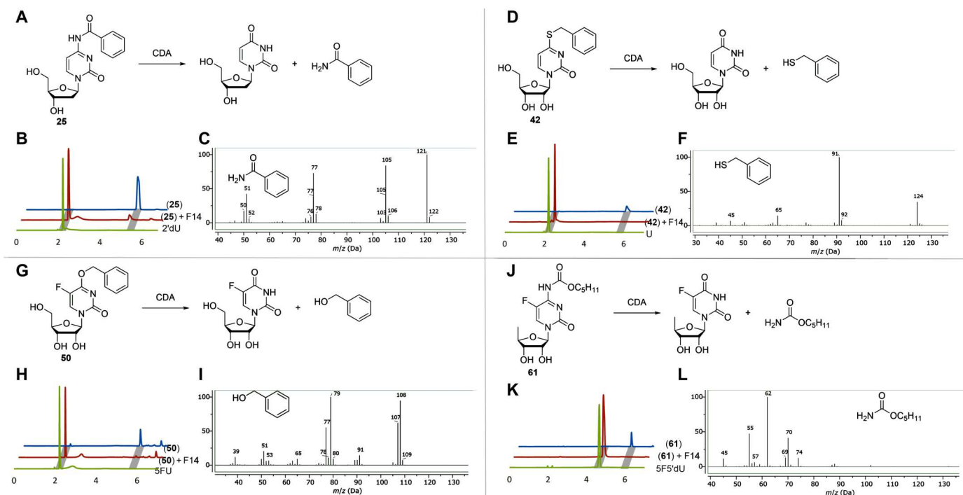
Fig. 1. A diversity of reactions catalyzed by CDAs. The conversion of N 4 -benzoyl-2'-deoxycytidine (25) (A), S 4 -benzylthiouridine (42) (D), 4-benzylthio-5-fluoro-uridine (50) (G), and capecitabine (61) (5'-deoxy-5-fluoro- N 4 -pentylloxycarbonylcytidine) (J) are shown. High-performance liquid chromatography–mass spectrometry chromatography spectra (254 nm) of reaction products: 2'-deoxyuridine (2'dU) (B), uridine (U) (E), 5-fluoro-uridine (5FU) (H), and 5-fluoro-5'dU (K), and typical GC-MS chromatography spectra outtakes of extracted reaction products: benzamide (C), benzyl mercaptan (F), benzyl alcohol (I), and pentyl carbamate (L) are shown after the reaction schemes, respectively. m/z , mass/charge ratio.
