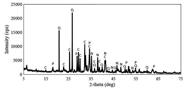
Figure 3. X-ray image of crystallising admixture: N – sodium carbonate ( \text{Na}_2\text{CO}_3 ), C – tricalcium silicate ( \text{Ca}_3\text{SiO}_4 ), Q – quartz ( \text{SiO}_2 ), P – portlandite ( \text{Ca}(\text{OH})_2 ).
