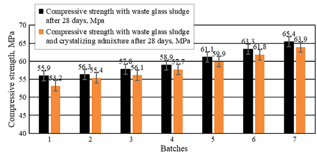
Figure 8. Compressive strength of hardened cement pastes with waste glass sludge and with waste glass sludge and crystallising admixture after 28 days.
