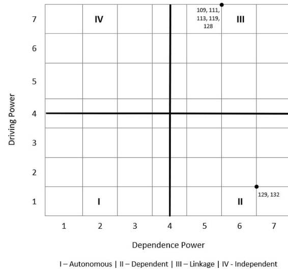
Fig. 6. C2 MICMAC and ISM diagram.
