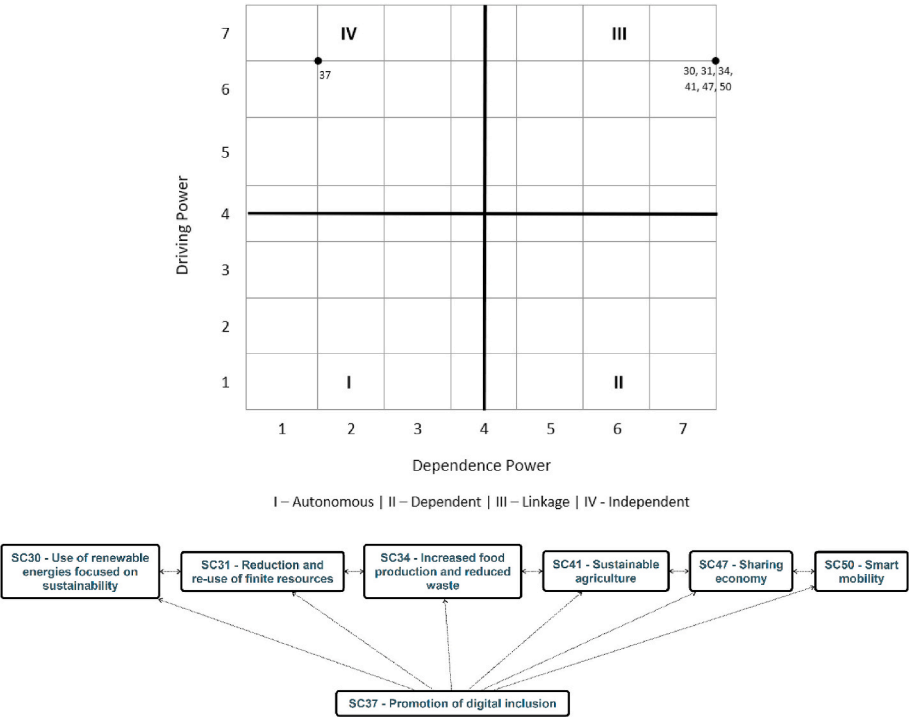
Fig. 5. C1 MICMAC and ISM diagram.
