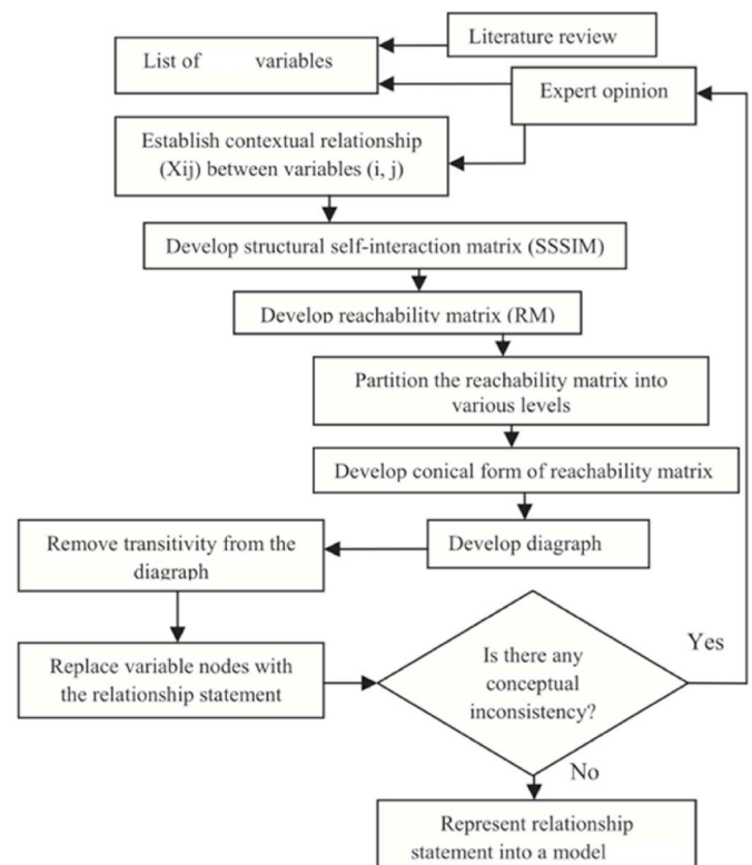
Fig. 2. Interpretive structural modeling steps.
