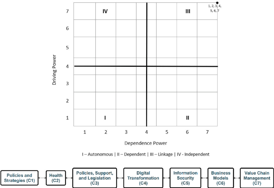
Fig. 4. Micmac and inter-cluster ISM diagram.
