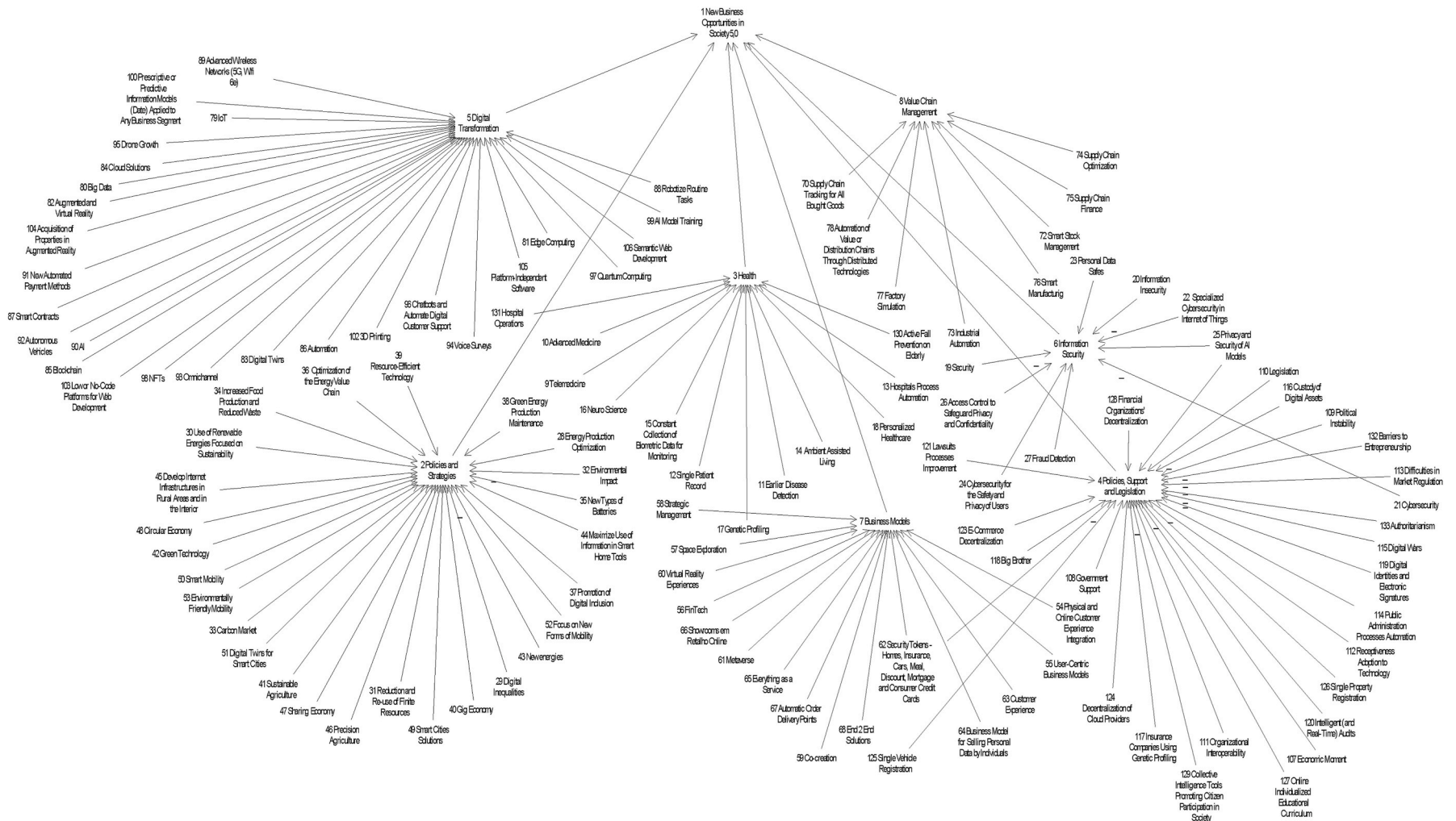
Fig. 3. Group cognitive map.
