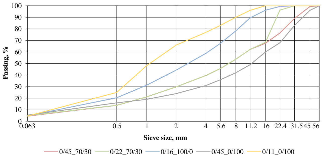
Figure 2. Particle size distribution of unbound mixtures used to construct a test road.
