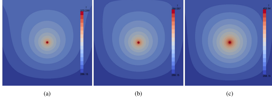
Figure 2. Distribution of temperature for different types of soil: (a) moist soil \lambda = 1.11 , (b) average soil \lambda = 0.83 , (c) dry soil \lambda = 0.41 .
