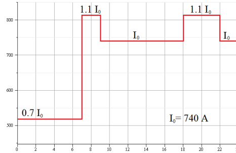
Figure 4. The daily dynamics of electrical currents.
