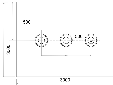
Figure 3. The layout of three cables in the soil.
