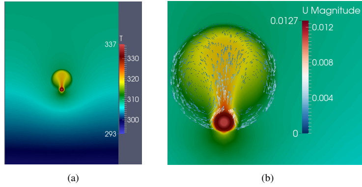
Figure 1. A single cable in a PVC tube: (a) distribution of temperature, (b) distribution of velocity fields.
