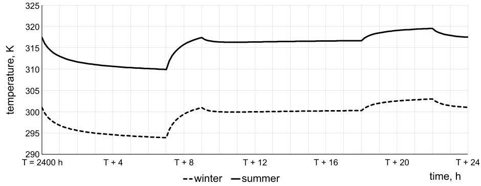
Figure 6. The daily dynamics of temperature for summer and winter cases.
