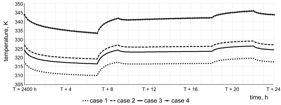
Figure 7. The daily dynamics of temperature for different placements of cables.
