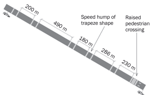
Figure 1 – Allocation of speed humps on the tested road section and picture of cameras used
