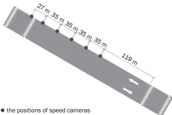
Figure 2 – The scheme of research on instantaneous speed
