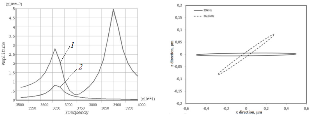
Fig. 3. Results of harmonic response analysis
