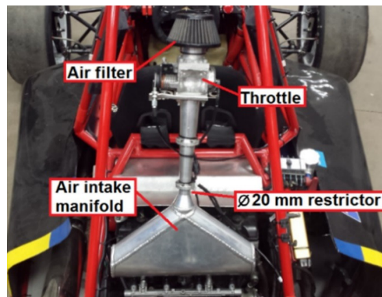
Fig. 2. Formula Student engine air intake manifold with Ø20 mm air restrictor.
