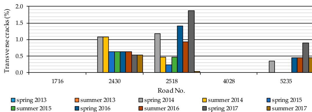
Figure 5. Transverse cracks on road sections covered with soft asphalt.
