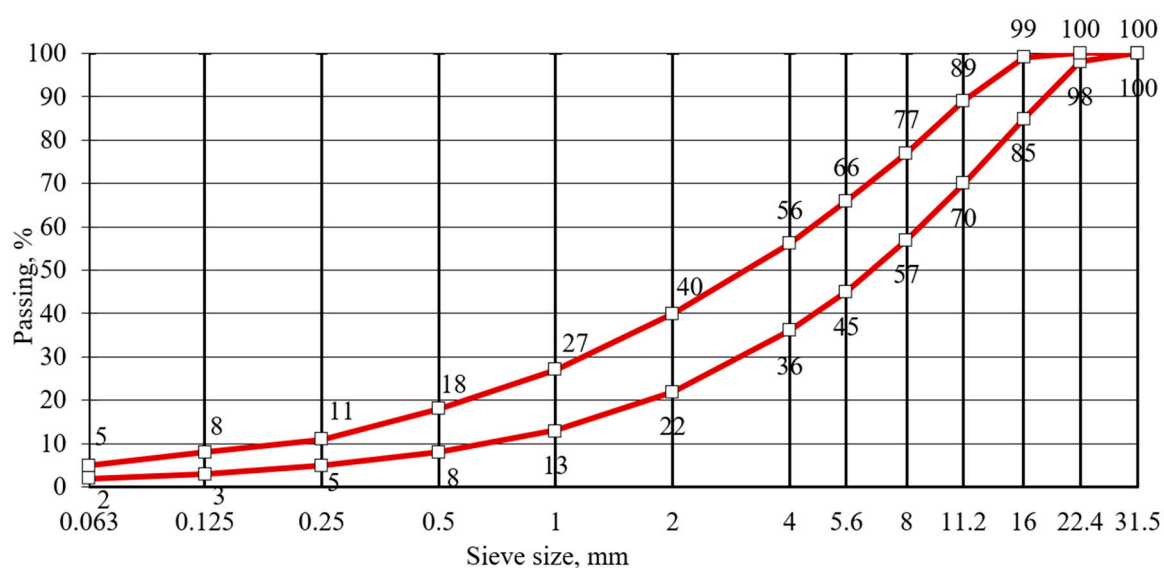
Figure 1. Aggregate gradation limits for double Otta Seal.
