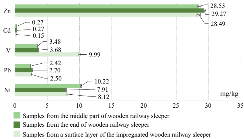
Figure 6. The concentration of heavy metals in a waste of the wooden railway sleeper
