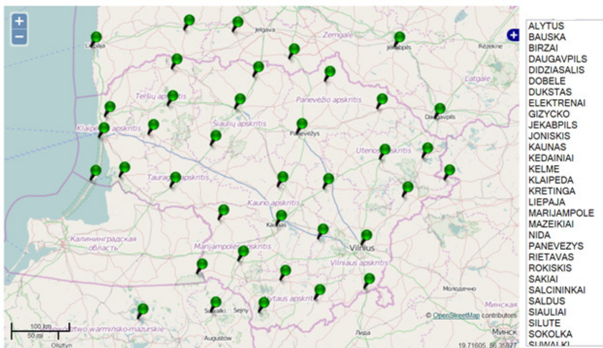
Fig. 1. LitPOS network map
