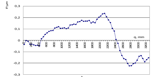
Fig. 4. Graphs of the correction measurements, evaluated by the active compensation method of the carriage's angular fluctuations about the horizontal axis (a) and the mean values thereof (b)
