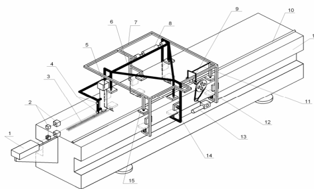
Fig. 1. The comparator's scheme with the main units and systems. 1- laser, 2- system of compensation Abbe errors in the vertical plane, 3- scale to be calibrated, 4- retroreflectors, 5- microscope with CMOS camera, 6- precise part of carriage, 7- powered part of carriage, 8- joint of carriage's parts, 9- friction wheel, 10- beam of friction gear, 11- joint of friction gear with carriage's parts, 12- belt gear, 13- gear-motor, 14- springy aerostatic bearing, 15- rigidly mounted aerostatic bearing, 16- granite basis with the guide-ways
