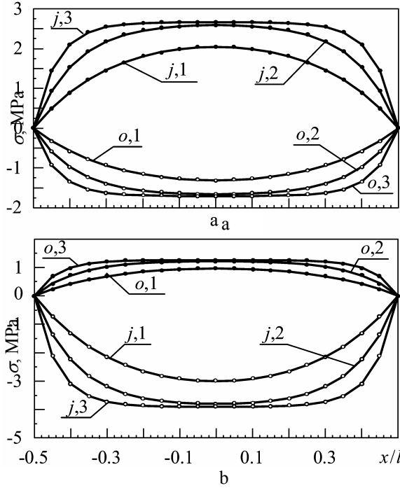
Fig. 4 Change of the layers' normal stresses through a beam length: a – in the first layer, b – in the second layer, j – at the joint of layers, o – on the outside of the layers, 1 - l=3 m, \xi=81 N/m; 2 - l=6 m, \xi=81 MN/m; 3 - l=6 m, \xi=270 MN/m, the parameters of the beam are given in Table
