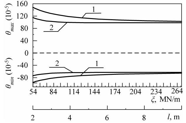
Fig. 6 Dependence of minimum \theta_{min} and maximum \theta_{max} thermal and hygral strain which does not induce the crack in the layers, on joint stiffness \xi when l=3 m – 1 and the length of beam l=2 , when \xi=54 MN/m, the parameters of the beam are given in the Table
