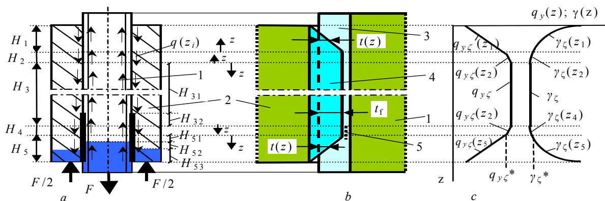
Fig. 1 Threaded joint divided into segments: a – segments, b – evolute of engaged turns, c – turns' deformation characteristics, 1 – stud; 2 – nut; 3 and 4 – evolutes of engaged stud and nut turns; 5 – cracks
