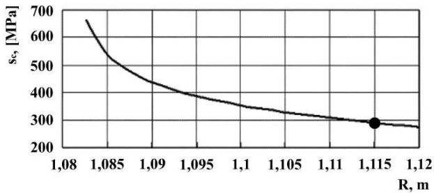
Fig. 7. The simulated maximum contact stress s_c plot versus teeth meshing contact position (half pitch diameter R=1.115 m)
