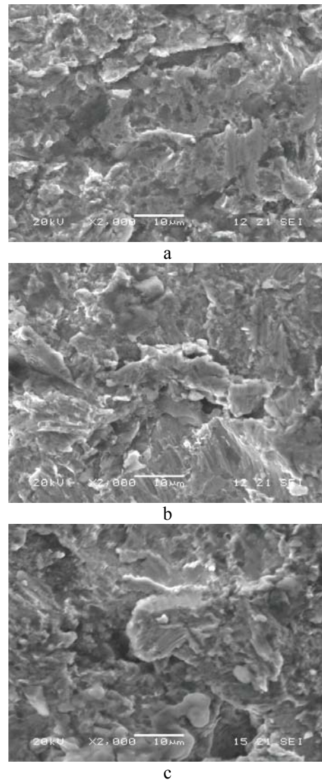
Fig. 8 SEM images of the layers affected by abrasive erosion wear at 90^\circ angle: a – sample 688, b – sample 682, c – reference Hardox 400
