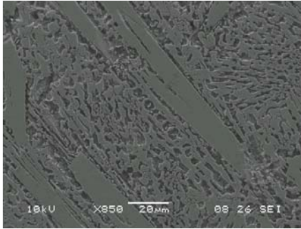
Fig. 3 Microstructure of welded layer (sample 674, SEM, ×850)
