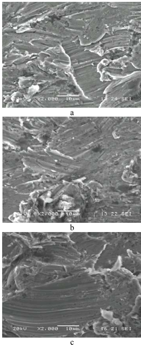
Fig. 7 SEM images of the layers affected by abrasive erosion wear at 30^\circ angle: a – sample 688, b – sample 682, c – reference Hardox 400
