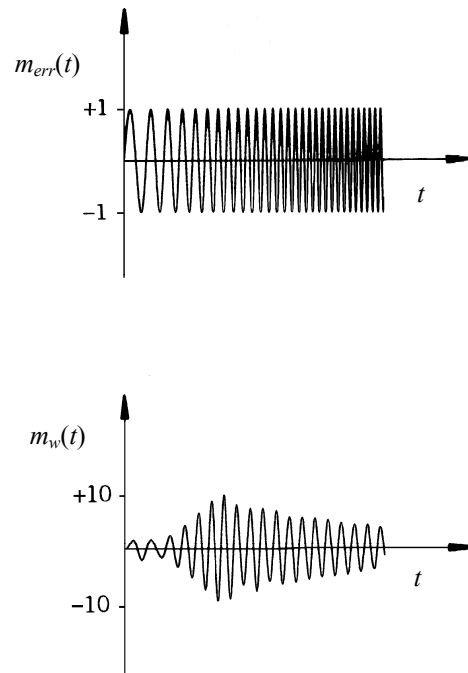
Fig. 1 Sweep function and excitation result
