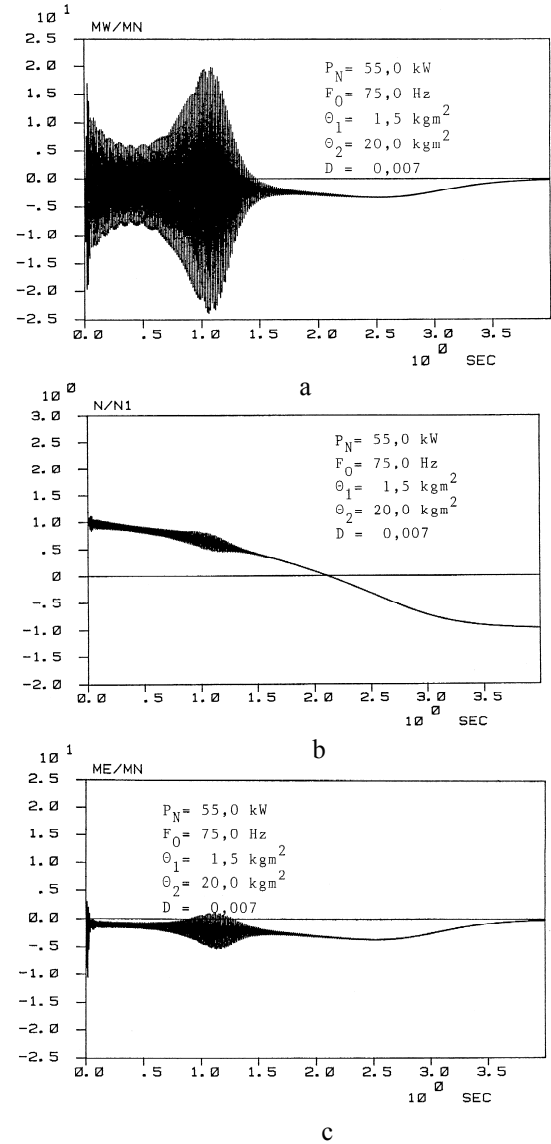
Fig. 5 a - parametric excitation of the shaft torque during reversal; b - simulation of the speed during reversal; c - simulation of electrical torque (reversal)
