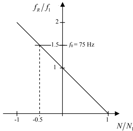
Fig. 7 Expanded excitation diagram
