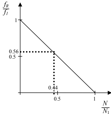
Fig. 4 Excitation condition diagram for run-up
