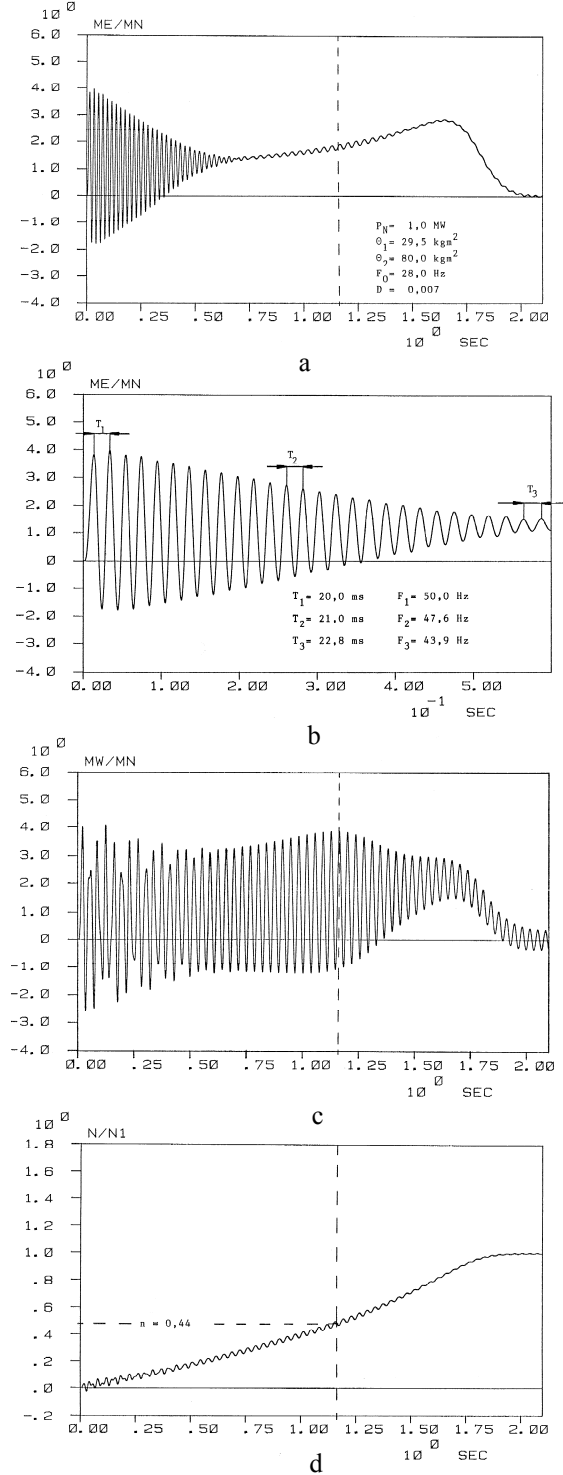
Fig. 3 a - simulation electrical torque (run-up); b - analysis of electrical torque after switch on; c - parametric excitation of the shaft torque (run-up); d - simulated speed (run-up)
