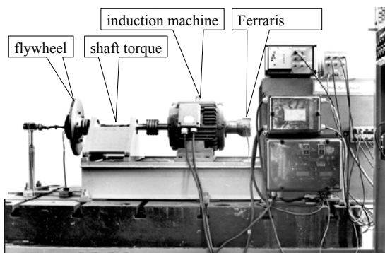
Fig. 8 Test rig to investigate torsional vibrations The motor is a 1.8 kW induction machine with
