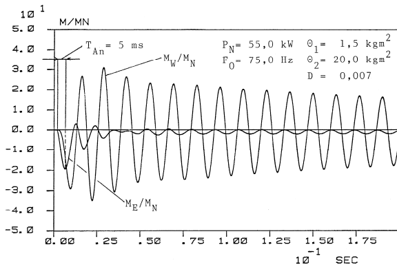
Fig. 6 Electrical impact and response of shaft torque at reversal switch
