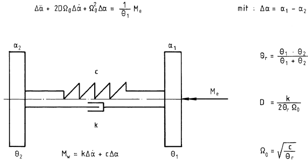
Fig. 2 Single degree-of-freedom torsional system
