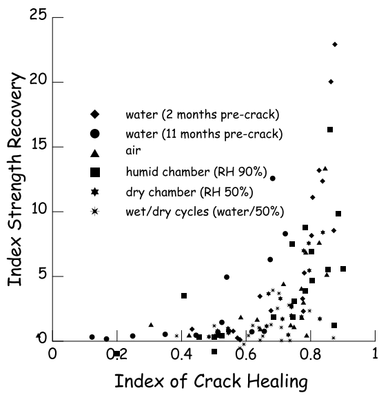
Fig. 10. Proposal for calculation of Index of Strength Recovery (a) and Index of Ductility Recovery (b) for strain hardening HPRC and correlation with Index of Crack Healing (c,d) [46,48].
