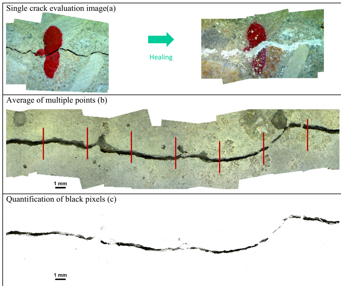
Fig. 4. Evaluation methods through evaluation of single cracks (a), average values of multiple points per specimen (b) and black pixels evaluation (c) [140,141].
