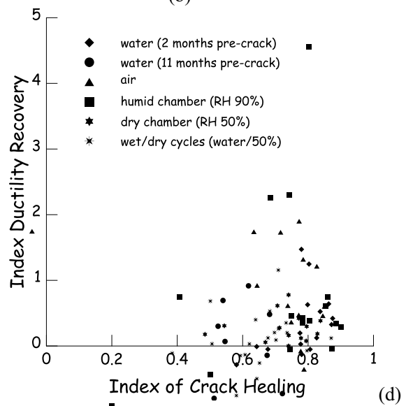
Fig. 10. Proposal for calculation of Index of Strength Recovery (a) and Index of Ductility Recovery (b) for strain hardening HPRC and correlation with Index of Crack Healing (c,d) [46,48].
