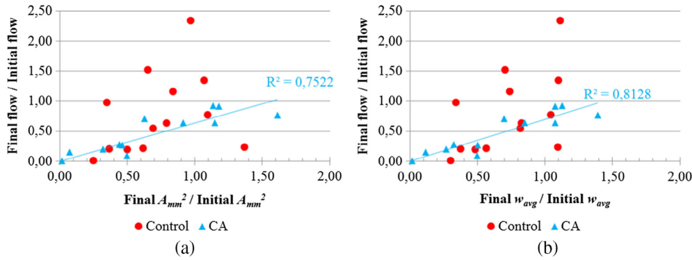
Fig. 7. 3-Relation between water flow ratio and estimated crack area A_{mn}^2 ratio (a) and averaged crack width w_{avg} ratio (b) for a control concrete mixture and a concrete containing crystalline admixtures (CA) from Roig-Flores et al. [140].
