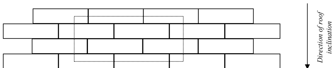
Fig. 1. Laying of 2000 × 600 mm magnitude roofing thermal insulating boards by overlapping joints
