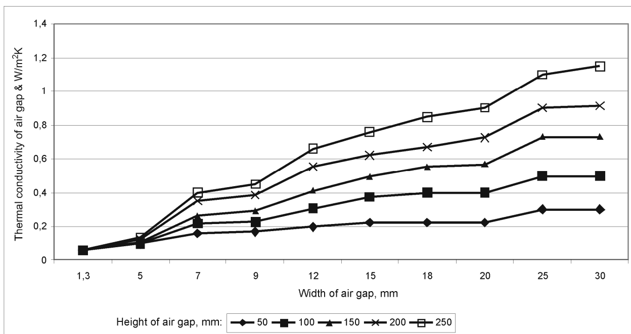
Fig. 3. The measured thermal conductivity values of vertical gaps of various widths and lengths
