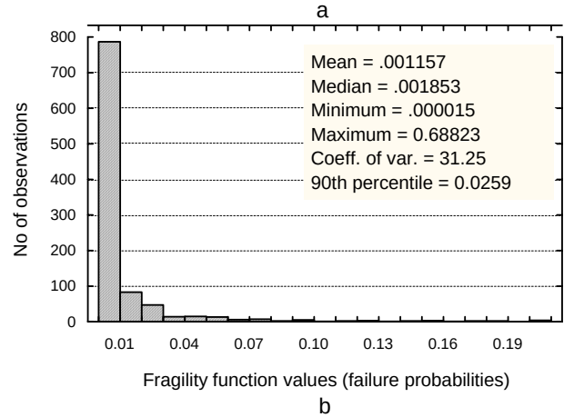
Fig. 4 Visualisation of the simulation results: a – histogram of the values of mean char depths d_{mj}(\boldsymbol{\theta}_{\beta k}) , b – histogram of the fragility function values p_j(\boldsymbol{\theta}_{\beta k})
