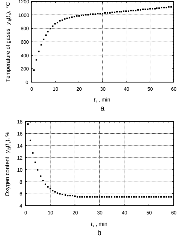
Fig. 2 Graphical representation of the realization y_j = \{(y_{1j}(t_\tau), y_{2j}(t_\tau)), \tau = 1, 2, \dots, 60\} of the signal y(t) ( \Delta t = 1 min): a – sequence of temperatures y_{1j}(t_\tau) , b – sequence of oxygen concentration y_{2j}(t_\tau)
