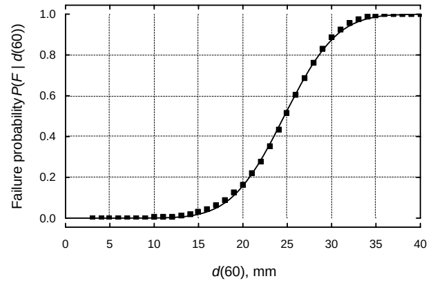
Fig. 3 Fragility function fitted to the estimated values of the conditional failure probability P(\mathcal{F} | d(60))
