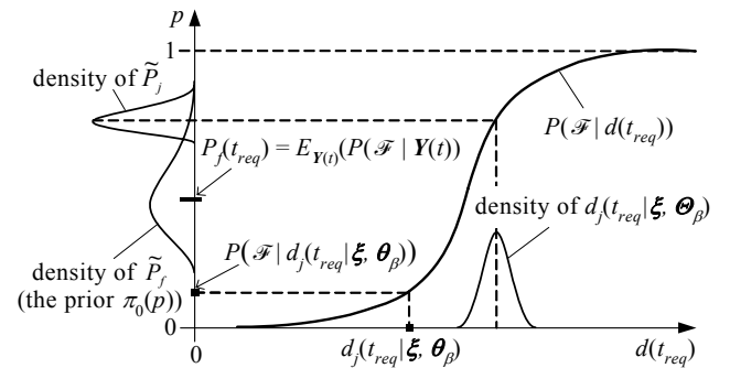
Fig 1 Fragility function values calculated for fixed char depths d_j(t_{req}) and uncertain char depths D_j(t_{req})
