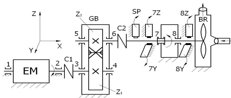
Fig. 1. The air blower machine scheme with proximity probes location: 1, 2 – journal bearings of EM; 3-6 – journal bearings of GB ( u = 0.477 , z_2 = 43 , z_1 = 90 ); 7, 8 – tilting-pad journal bearings of BR; C1, C2 – flexible couplings; 7Y, 7Z and 8Y, 8Z – proximity probes fixed at the 7 th and 8 th bearings, SP – keyphasor transducer
