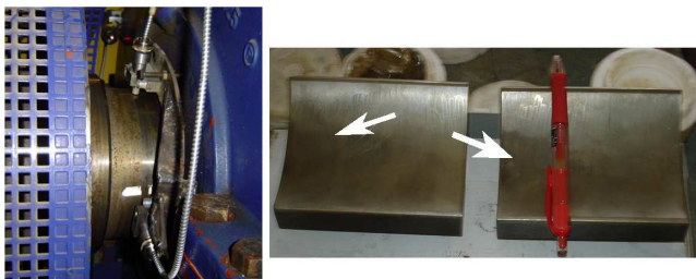
Fig. 2. The BR at 7 th bearing vibration displacements peak-to-peak values s_{p-p7Z} , s_{p-p7Y} and gaps-radial clearances \Delta 7Y , \Delta 7Z measurement set with two sensors 7Z and 7Y and damaged pads
