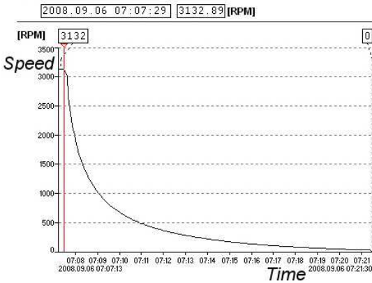
Fig. 4. The rotational speed timebase plot at coast down, time 841 s
