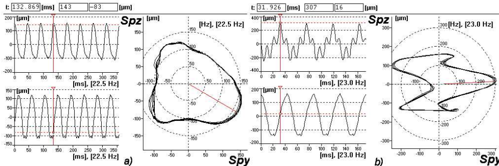
Fig. 6. The vibration displacement plots and kinetic orbits: a) 7 th bearing at resonance rotational speed, S_{max7rez} = 165 \mu m , s_{p-max7Zrez} = 250 \mu m , s_{p-max7Yrez} = 240 \mu m ; b) 8 th bearing at resonance rotational speed, S_{max8rez} = 307 \mu m , s_{p-max8Zrez} = 550 \mu m , s_{p-max8Yrez} = 300 \mu m
