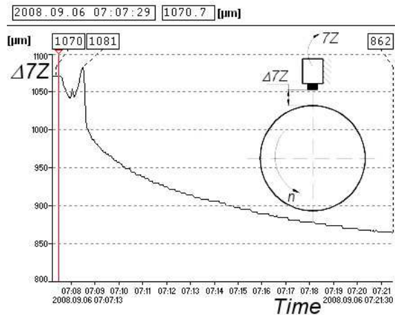
Fig. 7. The 7 th bearing vertical direction gap \Delta 7Z plot versus time at coast down: nominal gap decreased – 208 \mu\text{m} at 3119 rpm; resonance gap – 219 \mu\text{m} at 1350 rpm and reference position 862 \mu\text{m} at stand still, at 0 rpm
