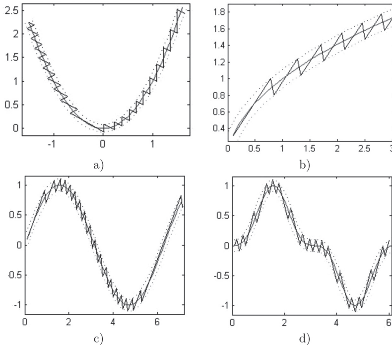
Fig. 3. Mobile piezorobot movement trajectory.
