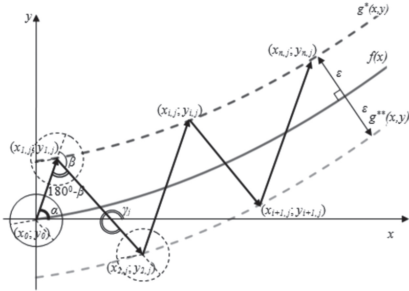
Fig. 2. Mobile piezorobot motion trajectory by given function f(x) .
