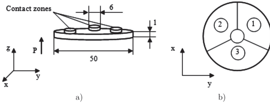
Fig. 1. Construction of mobile piezorobot.
