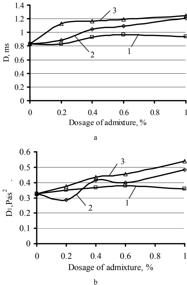
Fig. 11. Dependence of dilatancy rates D (a) and D_1 (b) on different amounts of plasticizing admixtures in Portland cement paste: 1 – with L plasticizer; 2 – with SNF superplasticizer; 3 – with PP superplasticizer
