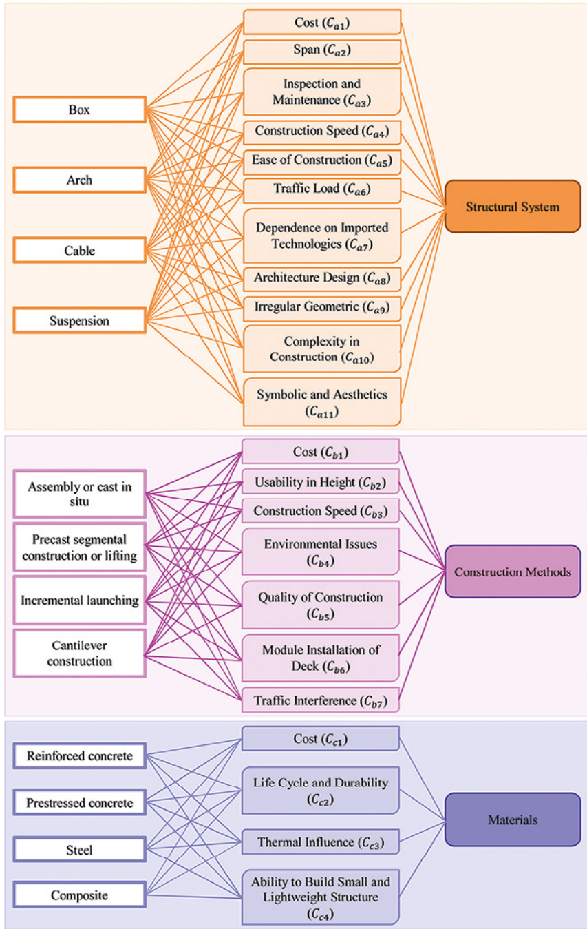
Figure 3. The hierarchical structure of the problems
