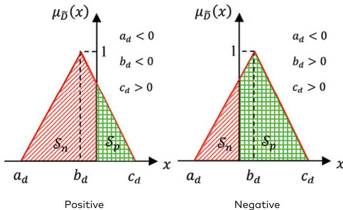
Figure 2. The graphical representation of Area-Based Deviation in two circumstances
