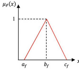
Figure 1. A Triangular Fuzzy Number
