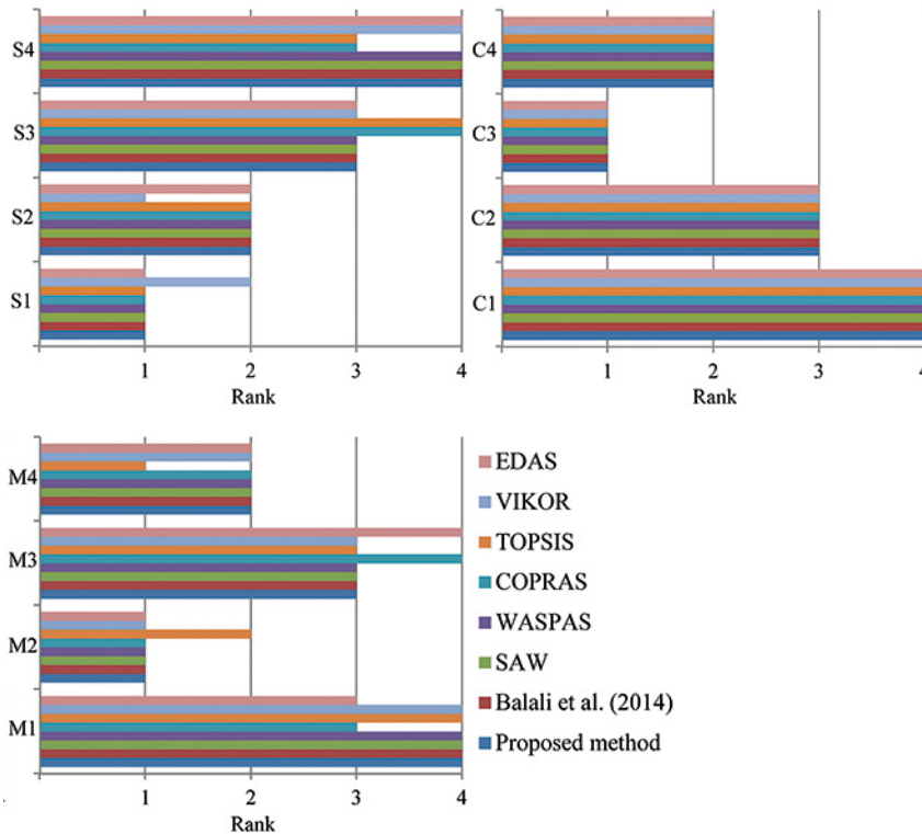
Figure 4. The graphical representation of the comparative analysis
