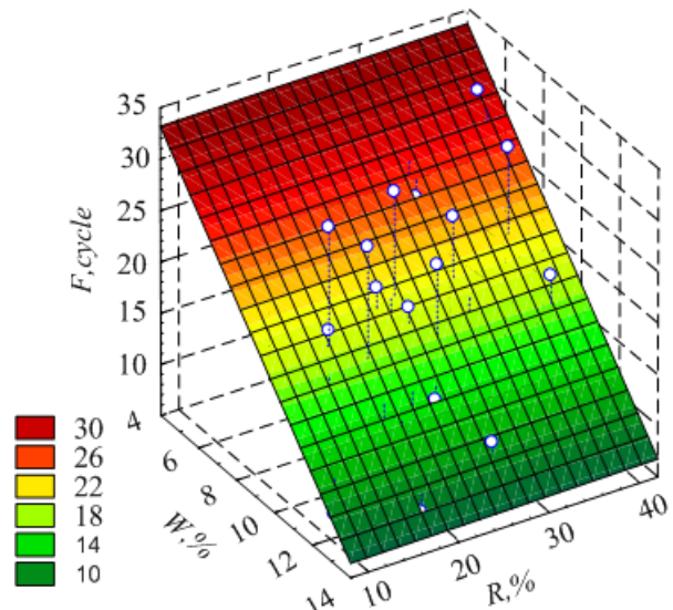
Fig. 6. Tendency of relationship between reserve of pore volume, water absorption and frost resistance determined by one-side method of freezing-thawing
