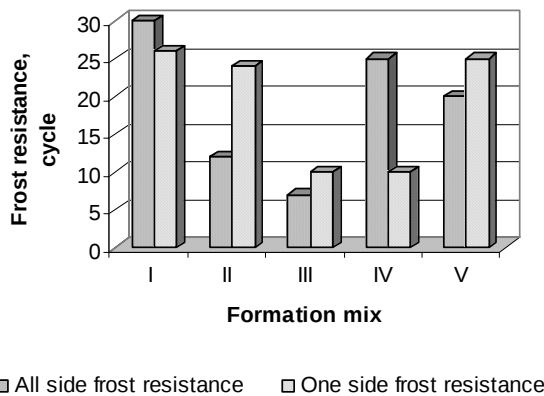
Fig. 4. Frost resistance of ceramic bodies measured by all-side and one-side method of freezing-thawing
