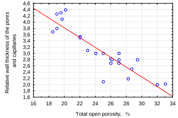
Fig. 2. Ceramic bodies dependence of relative wall thickness of the pores and capillaries on the total open porosity
