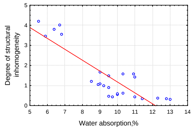
Fig. 3. Ceramic bodies dependence of water absorption on the degree of structural inhomogeneity
