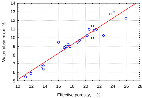
Fig. 1. Ceramic bodies dependence of water absorption on the effective porosity
