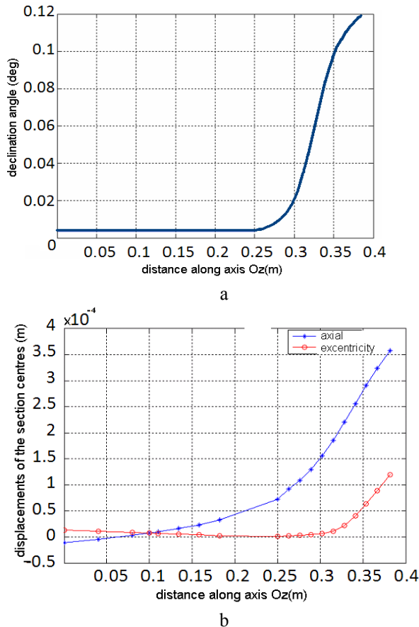
Fig. 3 Microscope with CCD camera fixed on its side: declination angle of symmetry axis (a), displacements of section centres (b)
