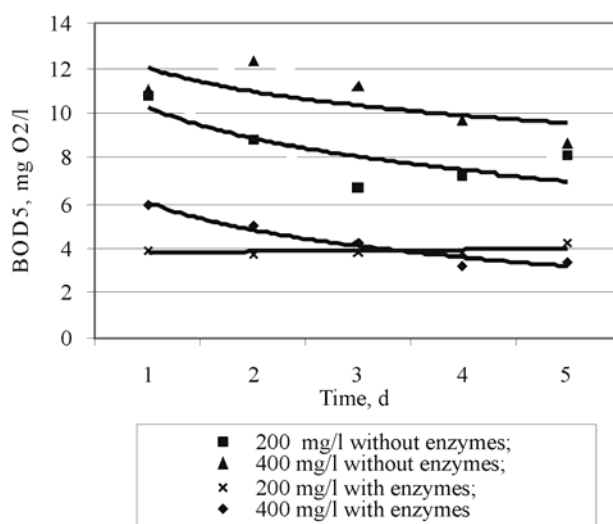
Fig. 1. Dependence of biochemical oxygen demand upon chloride concentration
