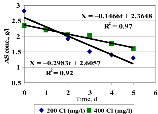
Fig. 3. Dependence of activated sludge concentration dynamics upon chloride concentration with enzymes
