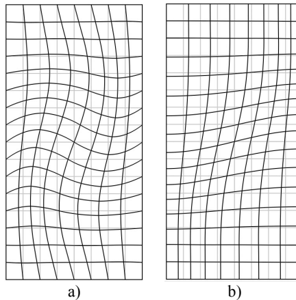
Fig. 4. The fourth eigenmode: a) elastic structure, b) fluid
