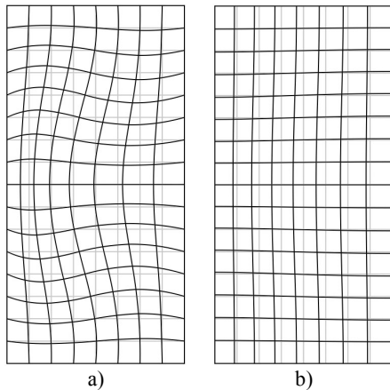
Fig. 3. The third eigenmode: a) elastic structure, b) fluid
