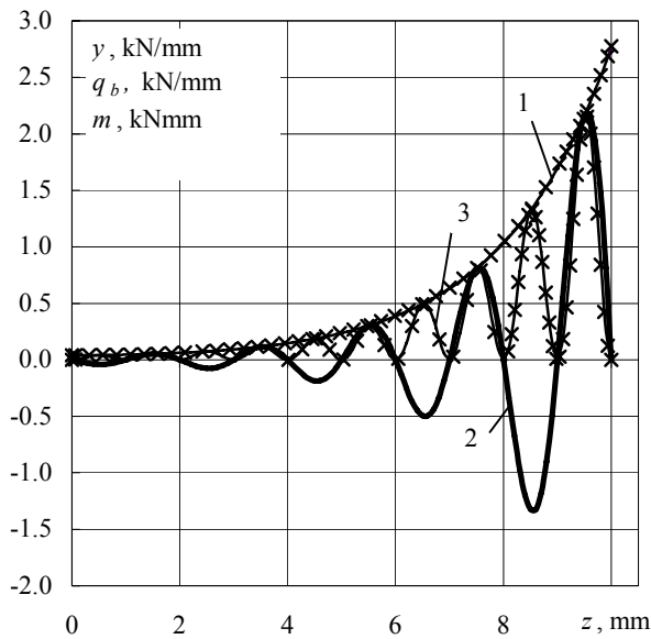
Fig. 4 Loads distribution in bent threaded joint M16: analytical solutions: 1 - y(z) , 2 - q_b(z) , 3 - m(z) ; x - numerical solutions
