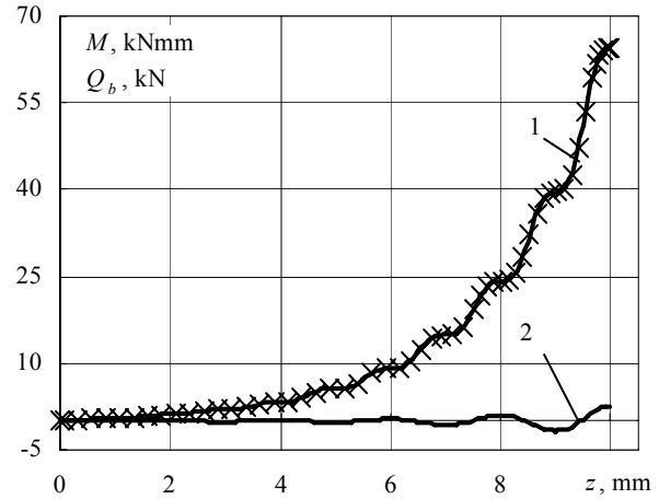
Fig. 5 Bending moment in the threaded joint M16: analytical solutions: 1 - M(z) , 2 - Q_b(z) ; x - numerical solutions
