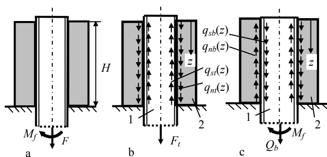
Fig. 1 Loads in threaded joint at bending: a – external loads, b – loads caused by tightening, c – loads caused by bending; 1 - stud, 2 - nut
