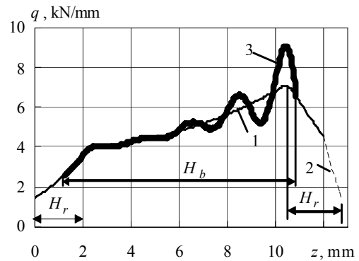
Fig. 6 Load distribution in the thread of tight stud at bending of the threaded joint M16: 1 - q_{st}(z) , 2 - q_{sb}(z) on plastically deformed part of runout, 3 - q_s(z) = q_{st}(z) + q_{sb}(z)
