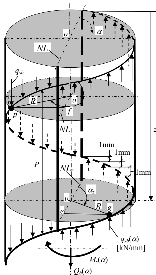
Fig. 2 Load intensity on helix turns of bended stud
