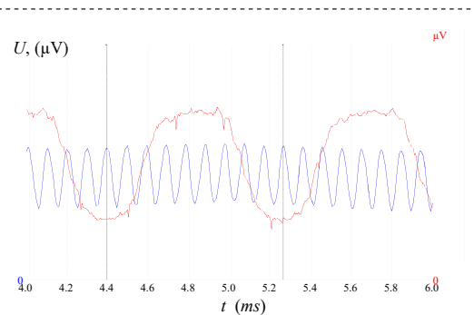
Figure 4. The signals of both reference encoder and a disk under test (lower frequency).
