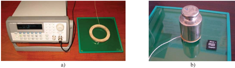
Fig. 2. Cases of increased load capacity: a) piezoelectric ring 140 \times 120 \times 8 mm ( D \times d \times h ), frequency – 80 kHz, voltage – 80 V; maximum weight of positioning object – 2 kg; b) piezoelectric ring 40 \times 10 \times 2 mm ( D \times d \times h ), frequency – 80 kHz, voltage – 50 V; maximum weight of positioning object – 500 g
