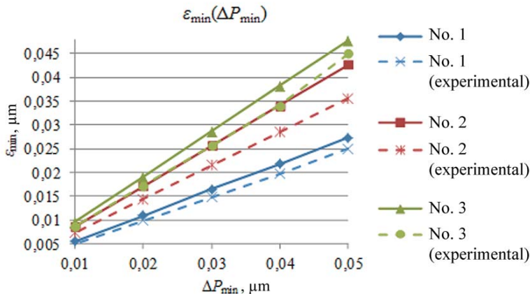
Fig. 10. The smallest deviation dependence on the motion resolution, when using switching contacts algorithm
