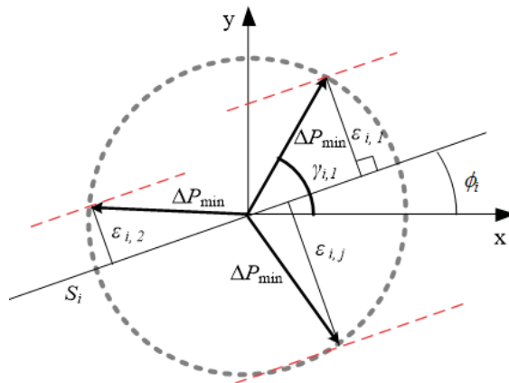
Fig. 5. Scheme of setting of minimum deviation from given trajectory
