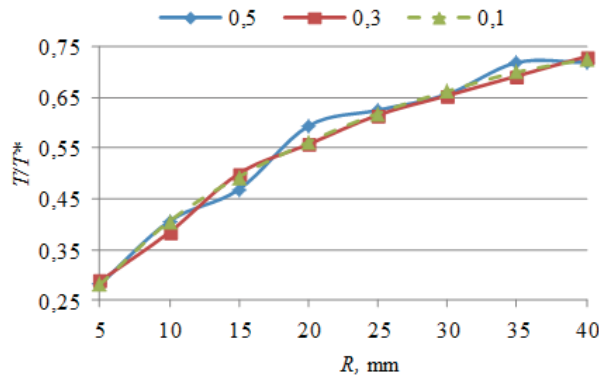
Fig. 12. Generated trajectory switching contacts quantity and control point's quantity ratio dependence on inner radius of piezorobot
