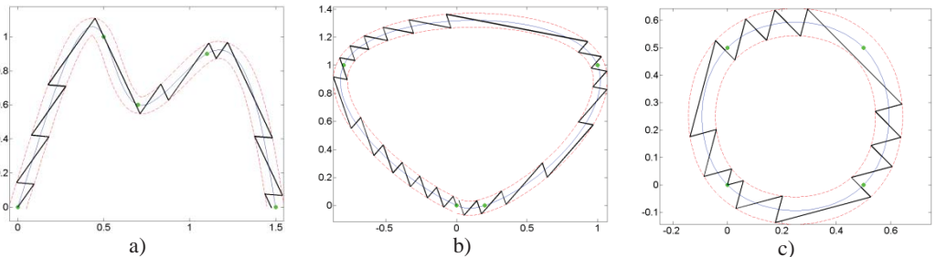
Fig. 8. Curves and generated micro-robot motion trajectories with switching contacts method: a) No. 4; b) No. 5; c) No. 6
