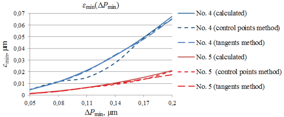
Fig. 11. The smallest deviation dependence on the motion resolution, when using control point's algorithm and tangents algorithm
