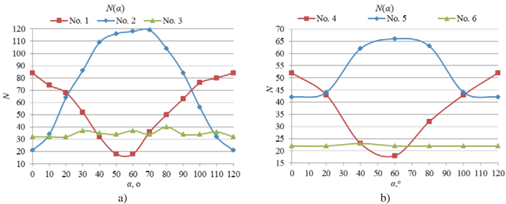
Fig. 9. Experimentally established dependencies of orientation angle of micro-robot, when given trajectories are: a) broken lines; b) curves
