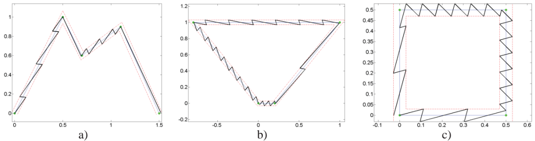
Fig. 7. Given broken line and generated micro-robot motion trajectories with switching contacts method: a) No. 1; b) No. 2; c) No. 3
