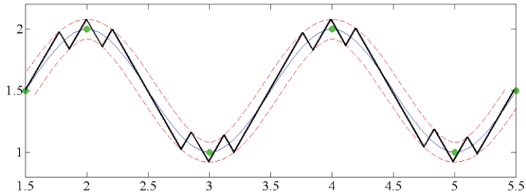
Fig. 3. Example of motion trajectory formation with switching contacts method
