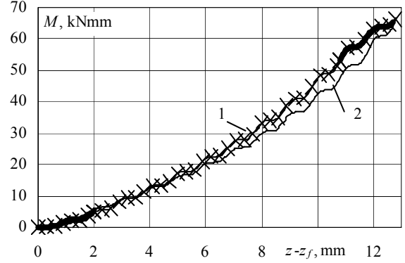
Fig. 7 Bending moment distribution in threaded joint M16×2 in position I: 1 – with estimating of runouts, 2 – model without runouts, lines – analytical solutions, × – numerical solutions of Eqs. (10 and 12)
