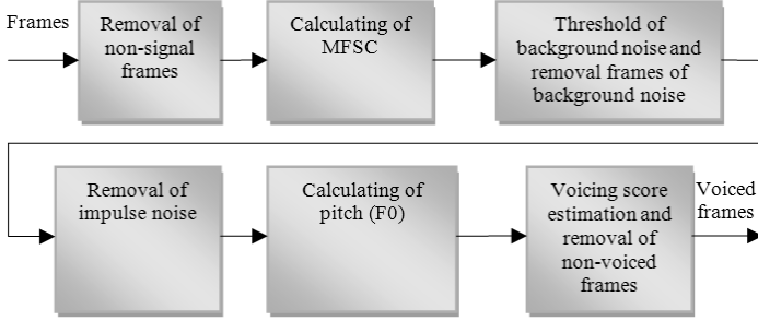
Fig. 2. Voice activity detection algorithm
