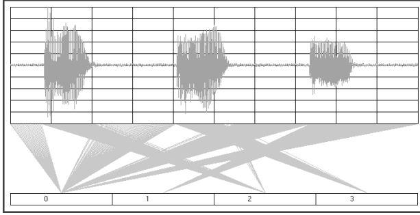
Fig. 6. Clusterization process
